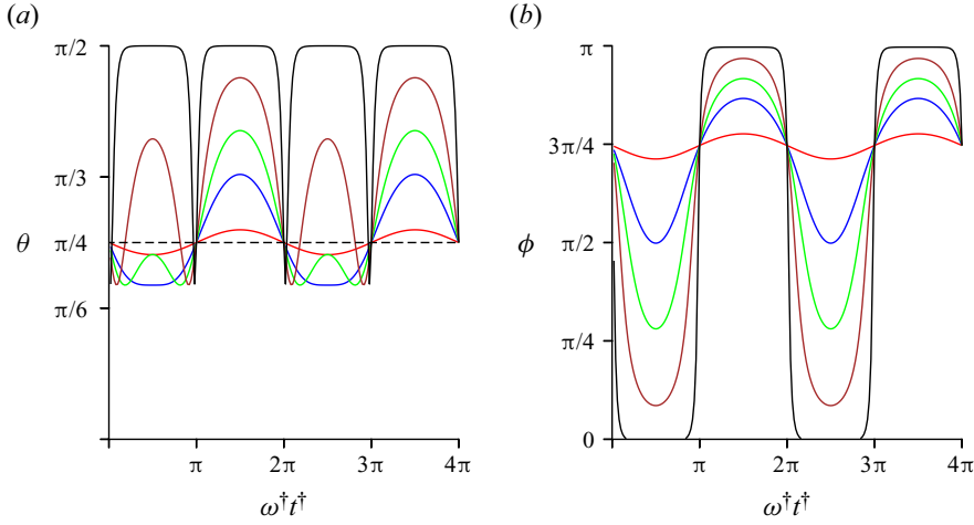
Figure 23. The variation of the angles \theta (a) and \phi (b) with scaled time \omega^+ t^+ for initial condition \theta = (\pi/4) and \phi = (3\pi/4) for \omega^+ = 10, 1.83, 1, 0.5, 0.1 .
