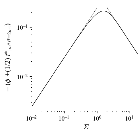
Figure 21. The variation of -(\phi + \frac{1}{2}t^*)|_{\omega^* t^* = 2n\pi} with the parameter \Sigma for \omega^* = 0.5 . The dashed black line on the left is the analytical result \frac{1}{4}\Sigma consistent with (4.20) and the dashed black line on the right is 0.5/\Sigma .
