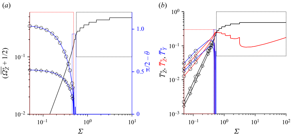
Figure 4. The variation in (a) (\bar{\Sigma}_Z^* + \frac{1}{2}) (black line) and \pi/2 - \bar{\theta} (blue line) and (b) \bar{T}_Z^* (black line), \bar{T}_Z^* (red line) and \bar{T}_Y^* (blue line) with the parameter \Sigma for \omega^* = 0.02 . The red, black and blue rectangles are expanded in figures 6, 10 and 12, respectively. Detailed analyses of the dynamics for the parameter regimes in the red, black and blue rectangles are carried out in §§ 5.1.1, 5.1.2 and 5.1.3, respectively. The initial conditions are \phi = 0 and \theta = (\pi/3) ( \circ ) and \theta = (\pi/6) ( \diamond ).
