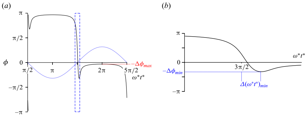
Figure 7. The time variation of the meridional angle \phi of the orientation vector for \omega^* = 0.02 and \Sigma = 5 , at the point P4 in figure 2. The dotted blue line in (a) is proportional to the scaled magnetic field, \cos(\omega^* t^*) . The blue rectangle in (a) is expanded in (b). The motion of the particle orientation vector on the unit sphere is shown in supplementary movie 2.
