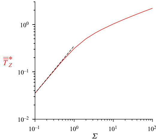
Figure 19. The variation in \bar{T}_Z^* with the parameter \Sigma for \omega^* = 0.5 . The dashed black line is the analytical result (4.22) for \bar{T}_Z^* .
