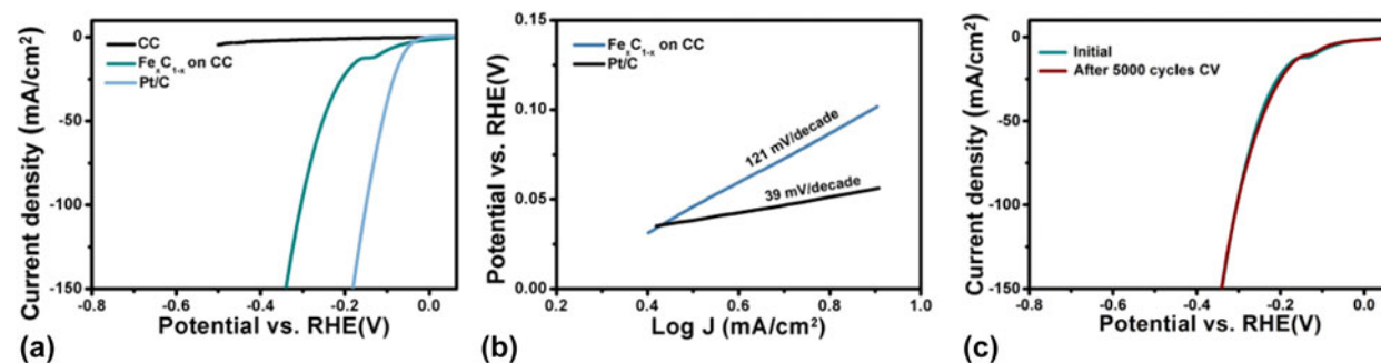
Figure 8: (a) LSV curves and (b) Tafel plots of the PEALD \text{Fe}_{1-x}\text{C}_x/\text{carbon cloth} and state-of-art Pt/C catalysts. LSV curve of bare carbon cloth is also included for comparison. (c) Comparison of LSV curves for PEALD \text{Fe}_{1-x}\text{C}_x/\text{carbon cloth} before and after 5000 cycles cyclic voltammetry.
