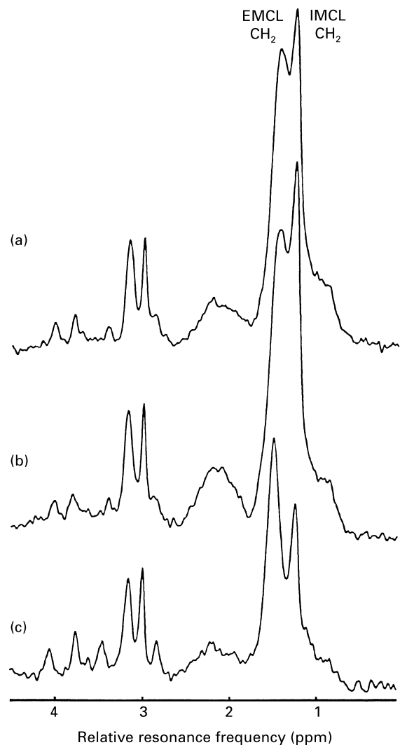
Fig. 2. 1 H-magnetic resonance spectra of three different types of skeletal muscle in the same volunteer at 2 d after a marathon run. Voxels of 11 × 12 × 18 mm 3 were located in (a) m. vastus intermedius , (b) m. vastus medialis and (c) m. tibialis anterior. The spectrum of m. tibialis anterior shows the best separation of the intramyocellular and extramyocellular lipids (IMCL and EMCL respectively) signals, due to the parallel orientation of the fat layers to the magnetic field (Boesch et al. 1997). The IMCL levels in the m. vastus are significantly higher than the one in the m. tibialis . ppm, Parts per 10 6 .
