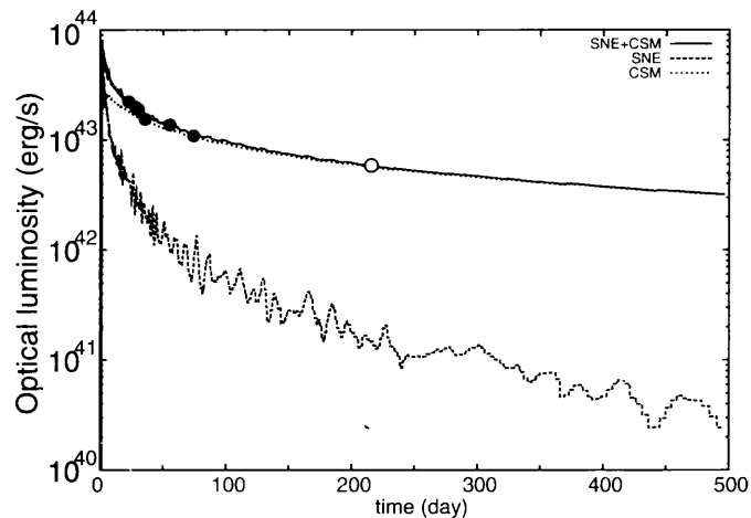
Fig. 1. Calculated light curve with observed data points (Subaru data point (Deng et al. 2003) is shown in open circle).
