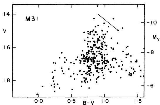
Fig. 3. Integrated CM diagram of M31 clusters
