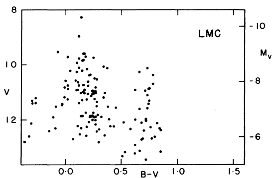
Fig. 2. Integrated C-M diagram of the LMC clusters
