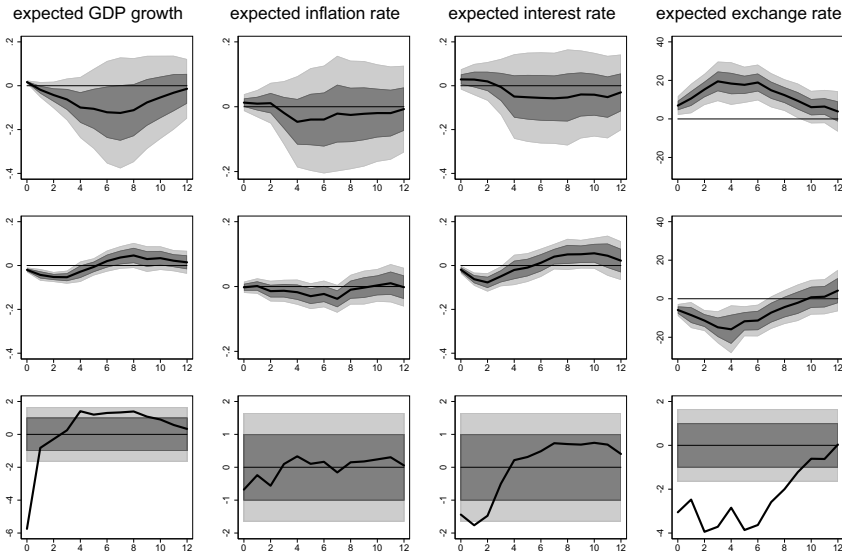
Figure 5. Responses of expectations to global uncertainty conditional on exchange rate stability. Notes: The figure shows impulse response functions of the survey measures. In each panel, the upper panels show responses of expected growth rates where the policy choice is evaluated at 0 and at 1 in the middle panel. The lower panels show t-statistics on the difference between responses. See also notes in Figure 2.
