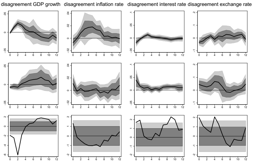
Figure 9. Responses of disagreement to global uncertainty conditional on monetary independence. Notes: The figure shows impulse response functions of the survey measures. In each panel, the upper panels show responses of expected growth rates where the policy choice is evaluated at 0 and at 1 in the middle panel. The lower panels show t-statistics on the difference between responses. See also notes in Figure 2.
