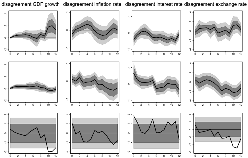
Figure A.8. Responses of disagreement to global uncertainty conditional on monetary independence (GEMu). Notes: The figure shows impulse response functions of the survey measures to a one-standard deviation surge in the uncertainty measure by Baker et al. (2016). In each panel, the upper panels show responses of expected growth rates where the policy choice is evaluated at 0 and at 1 in the middle panel. The lower panels show t-statistics on the difference between responses. See also notes in Figure 2.
