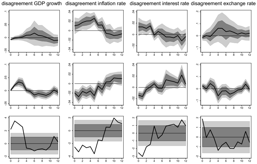
Figure 8. Responses of disagreement to global uncertainty conditional on exchange rate stability. Notes: The figure shows impulse response functions of the survey measures. In each panel, the upper panels show responses of expected growth rates where the policy choice is evaluated at 0 and at 1 in the middle panel. The lower panels show t-statistics on the difference between responses. See also notes in Figure 2.
