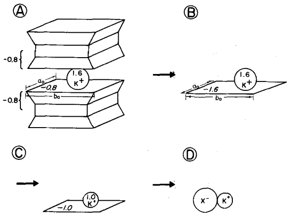
Figure 1. Derivation of Eq. (6) for an illite-like example (depicted in A) which has a layer charge (C) of -0.8 equivalents per O_{10}(OH)_2 and an ab unit cell area on each interlayer surface of A. In B the upper interlayer surface in A has been superimposed on the lower surface, yielding a plane with half the surface area of the two planes in A, but with twice the charge of an ab plane. This situation is energetically equivalent to that shown in A because energy is a scalar quantity. In C the surface areas of the plane and cation are adjusted proportionately until the charge on each is -1 and +1 respectively. The new area ( A' ) of the plane equals -A/2C . In D the negative plane has been transformed into an electrically equivalent sphere. The electric field strength ( E ) of a surface is given by E = 4\pi\sigma k , where \sigma is the surface charge density (charge/surface area) and k is the constant of proportionality (Sears and Zemansky, 1955). Thus, for the sphere in D, E_s = qk/r^2 , where q is the charge and r the radius. For the plane in C, E_p = 4\pi kq/A' . Setting E_p equal to E_s and solving, r = (A'/4\pi)^{1/2} . Substituting in the relationship for A' given above yields the radius of the equivalent anion, r_a = (-A/8\pi C)^{1/2} .
