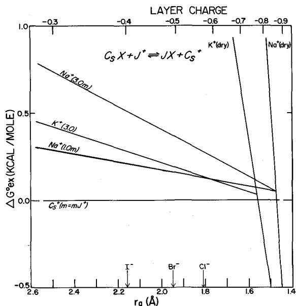
Figure 6. A comparison between Cs-K exchange at 3 molal and Cs-Na exchange at 3 molal and 1 molal.
