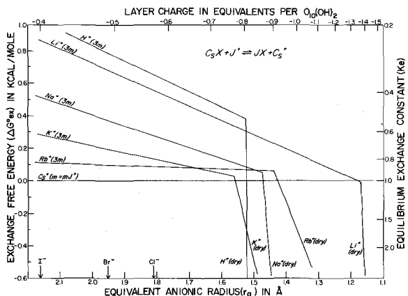
Figure 3. Change in exchange free energy ( \Delta G^{\circ}ex ) with r_a for the reaction indicated, where J^+ is an alkali cation. Calculations for smectite curves made for a 3 molal interlayer solution. The lowest curve is for the cation that is most preferred by the clay, and the separation between curves is a measure of how much it is preferred.
