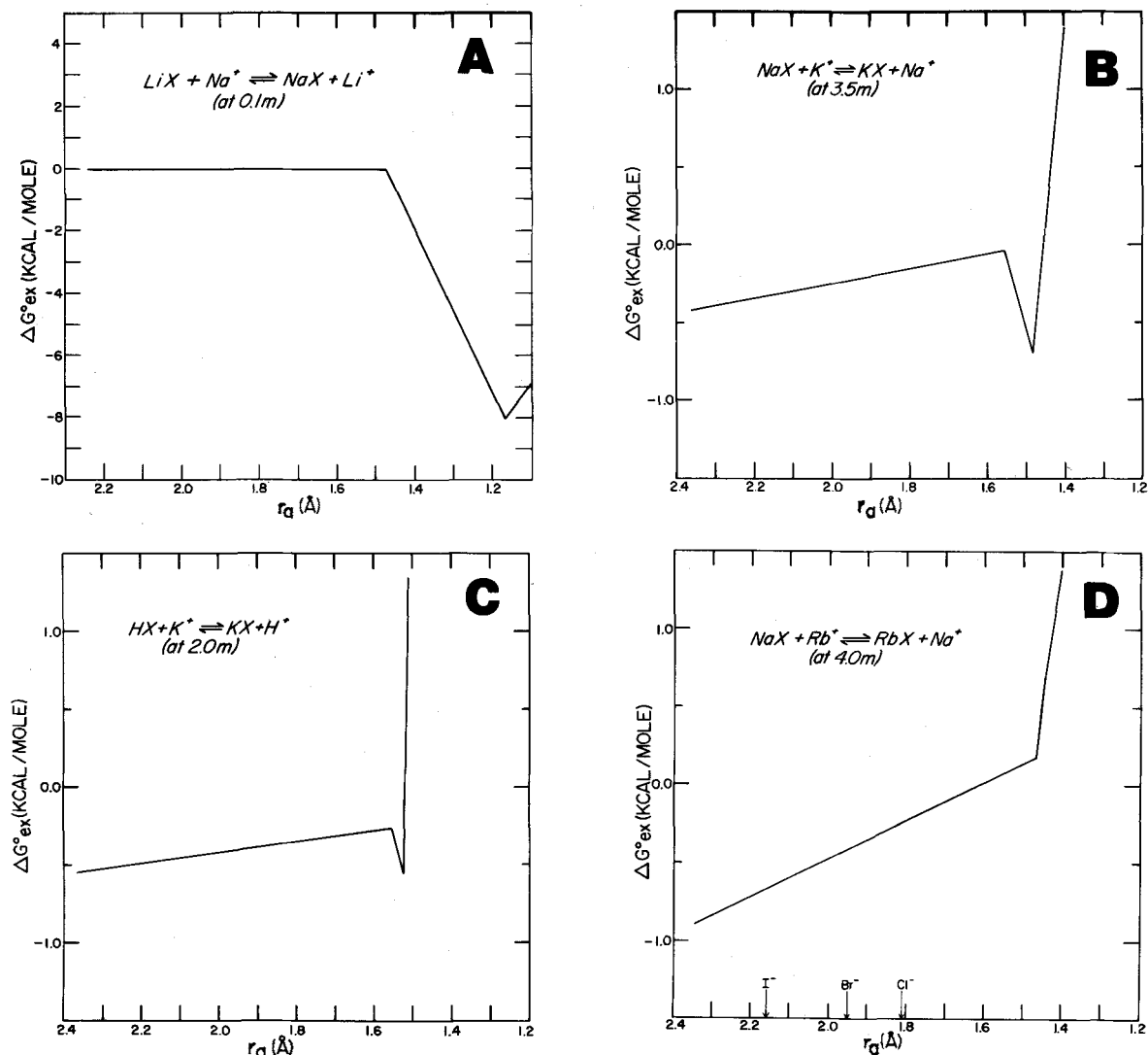
Figure 8. Calculated change in \Delta G^{\circ}\text{ex} with r_a for four exchange reactions. Molalities for A, B, and D are "best fit" molalities from Table 2. Molality for C was chosen arbitrarily.
