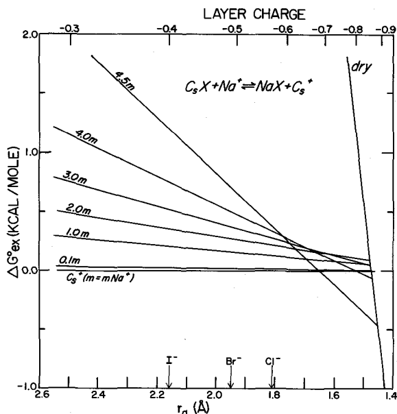
Figure 4. Change in \Delta G^{\circ}ex with r_a for the Cs-Na reaction indicated for several interlayer water contents.
