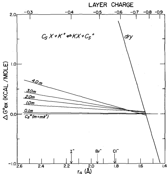
Figure 5. Change in \Delta G^{\circ}ex with r_a for the Cs-K reaction indicated for several interlayer water contents.
