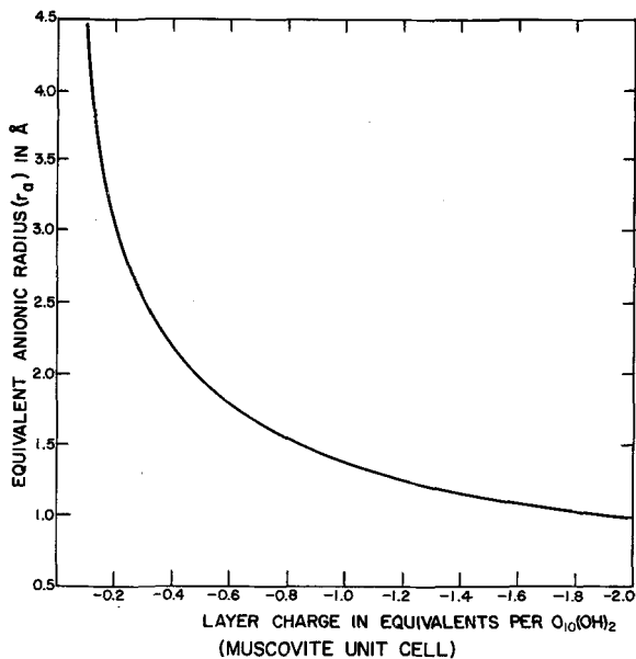
Figure 2. Relationship between equivalent anionic radius ( r_a ) and layer charge (using ab area of muscovite).
