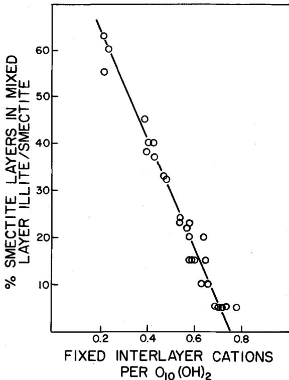
Figure 9. Percent smectite layers in mixed-layer illite/smectite vs. number of fixed cations in illite layers (from Hower and Mowatt, 1966).
