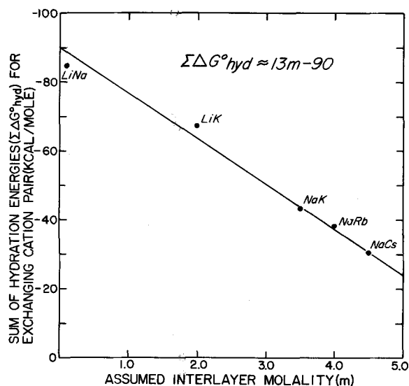
Figure 7. Sum of hydration energies for cations undergoing exchange plotted against "best fit" interlayer molalities from Table 2.
