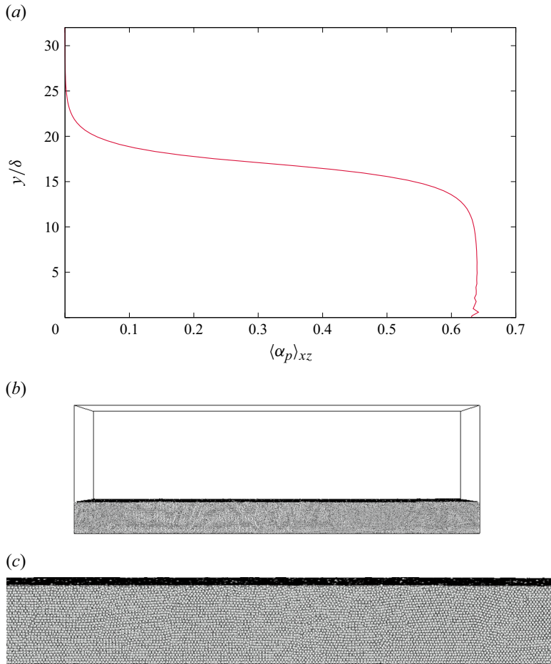
Figure 2. The particle bed is initialised by letting particles settle onto the bottom wall. (a) This procedure results in a volume fraction profile that is consistent with that of a poured bed. (b,c) The isosurface \alpha_p = 0.2 represents a good indicator of the location of the bed–fluid interface.
