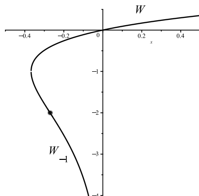
FIGURE 1. A branch of the Lambert W-function.
