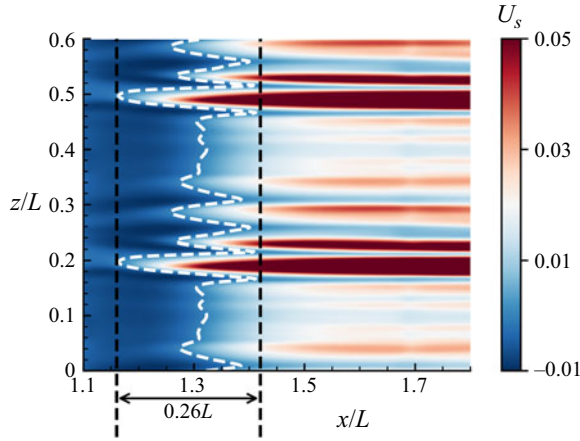
Figure 22. Instantaneous streamwise velocity distributions after being fully developed on the X - Z plane at y_n/L = 8 \times 10^{-5} with spanwise width 0.6L . The white dashed line is the reattachment line.
