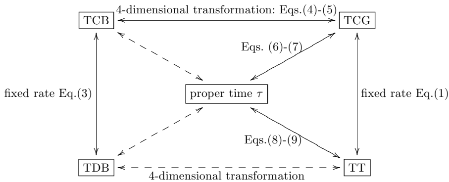
Figure 1. Various relativistic time scales and their relations. Each of the coordinate time scales TCB, TCG, TT and TDB can be related to the proper time \tau of an observer, provided that the trajectory of the observer in the BCRS and/or GCRS is known. See chapter 10 in the IERS Conventions web site at http://tai.bipm.org/iers/convupdt/convupdt.html for reference to the transformations listed in the Figure.
