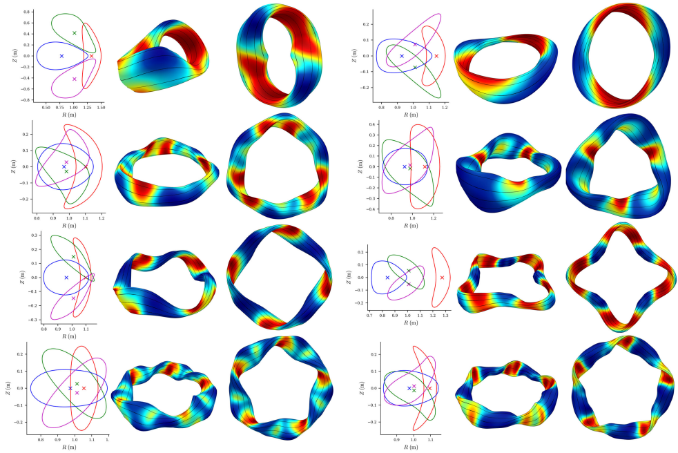
FIGURE 4. Examples of the equilibria generated with random boundary Fourier modes. Two-dimensional plots show the cross-sections at which the toroidal angle is 0, 1/4, 1/2 and 3/4 of a field period. Three-dimensional images show each configuration from two angles, with colour indicating |B| (red = high, blue = low) and field lines in black.
