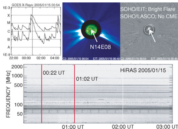
Figure 1. (Top) GOES soft X-ray flare, SOHO/LASCO image with superposed EIT image showing the flare and SOHO/LASCO and EIT difference images. (Bottom) Radio dynamic spectrum from the Hirasio radio spectrograph (HiRAS) with the start (00:22) and end (01:02) times of the flare marked. The flare of interest is pointed by arrows. Note that there is no radio emission during the flare.
