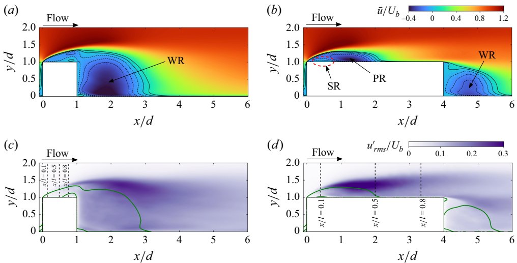
Figure 10. (a,b) Mean streamwise velocity ( \bar{u} ) contours overlaid with mean velocity streamlines; and (c,d) contours of root-mean-squared streamwise fluctuations ( u'_{rms} ) overlaid with streamline of \bar{u} = 0 . Contours presented for (a,c) DR = 1 and (b,d) DR = 4 prisms at Re = 2.5 \times 10^3 at spanwise plane of z/d = 0 .
