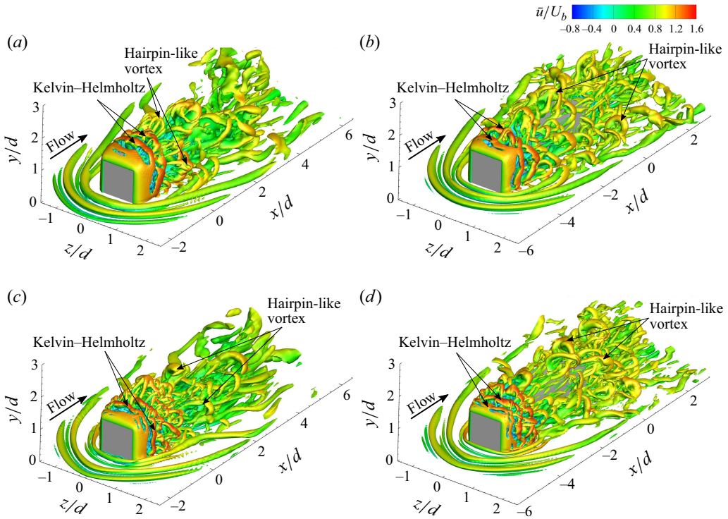
Figure 9. Instantaneous vortex structures overlaid with axial velocity ( u ) contours for (a,c) DR = 1 and (b,d) DR = 4 prisms at (a,b) Re = 5 \times 10^3 and (c,d) Re = 1 \times 10^4 , identified using Q -criterion ( Q^* = 1 ).
