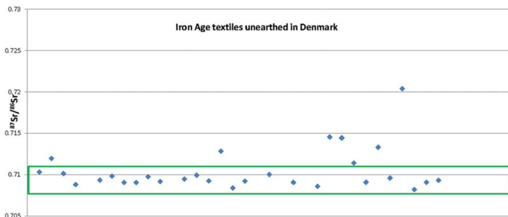
Figure 9. The strontium isotope results from wool samples from Early Iron Age bog textiles from Denmark corresponding to Table S2. The green rectangle shows the strontium isotopic range characteristic for Denmark (the island of Bornholm excluded).
