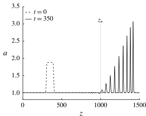
FIGURE 8. Initial (dashed) and final (solid) profiles for a numerical simulation of the conduit equation box problem ( a_m = 0.88 , w = 96 ) that results in nine solitary waves. The location z_* = 1000 separates the solitary wavetrain to the right from small-amplitude dispersive radiation.
