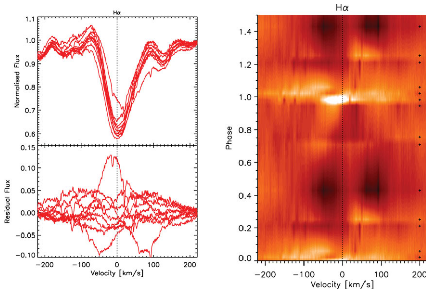
Figure 3. Left: All the H \alpha profiles from the UVES data. Upper plot shows the profiles normalised to the continuum, and the lower plot the residual profiles after subtracting the mean profile (thick line in the upper plot). Right: Dynamic spectrum of the H \alpha line based on the residual profiles. The x-axis gives the velocity and the y-axis the phase. The crosses on the right hand side of the plot give the phases of the observations and the dotted line the zero velocity. Brighter the colour the more emission is observed. The phases go from 0.0 to 1.5 to better show the flare occurring near the phase 0.0 (1.0).
