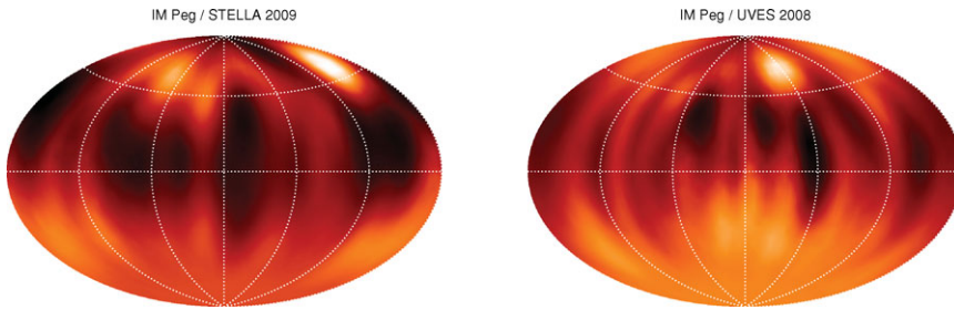
Figure 1. Temperature maps obtained from the UVES and STELLA data using Doppler imaging techniques and Fe I 6430 Å line.
