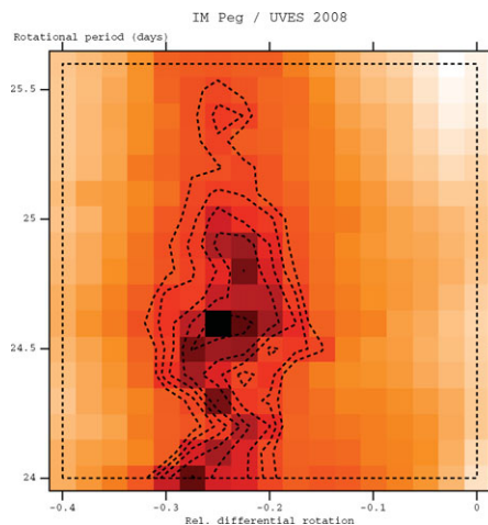
Figure 2. The goodness of fit parameter for the UVES dataset with varying period and differential rotation.
