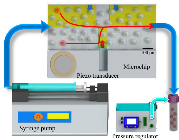
Figure 2. Microfluidic chip and its associated flow control system. The 20 mm microchannel features a rectangular cross-section ( H = 100\ \mu\text{m} \times W = 500\ \mu\text{m} ), with a central cavity measuring w = 80\ \mu\text{m} in width and h = 500\ \mu\text{m} in length. A syringe pump regulates the flow rate, while a piezoelectric transducer stimulates a microbubble, and a pressure regulator stabilises liquid and bubble pressures. A customised LabVIEW control system enables real-time cell detection and tracking, adjusting the piezoelectric transducer to guide cells along red pathways to a target region for collection. Regions of interest (ROIs) for cell detection are marked in yellow, with blue arrows indicating downward flow and a red arrow representing upward flow generated by microbubble activation.
