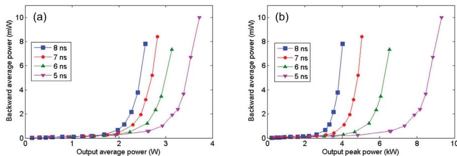
Figure 7. Average backward propagating power of square-like pulses as functions of the (a) average forward propagating output and (b) peak power.
