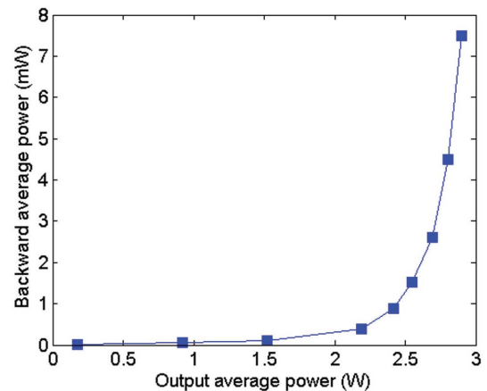
Figure 5. Average backward propagating power of the Gaussian-like pulses as a function of the forward propagating output power.
