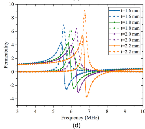
Figure 5. Effective permeability of the MM with different structure parameter variation: (a) turn of spiral N , (b) line width of spiral w , (c) line spacing of spiral s , and (d) thickness of substrate t .
