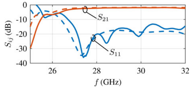
Fig. 13. Simulated (dashed line) and measured (solid line) results of the SIW-to-SIW transition in a back-to-back arrangement.
