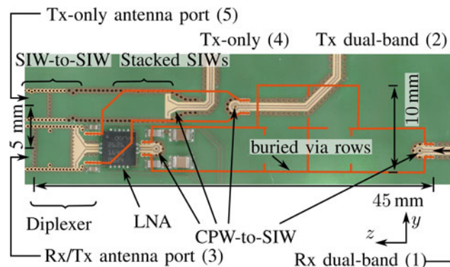
Fig. 18. Photograph of the frontend circuit for the interleaved array.
