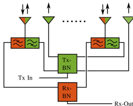
Fig. 2. Simplified frontend schematic representation of an antenna module.
