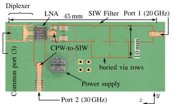
Fig. 15. Photograph of the manufactured dual-band element frontend.
