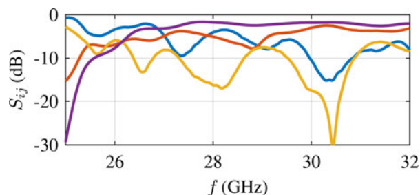
Fig. 19. Measured frontend performance. S_{22} (blue line) and S_{32} (red line) of the dual-band feed and S_{44} (yellow line) and S_{54} (purple line) of the Tx-only feed.
