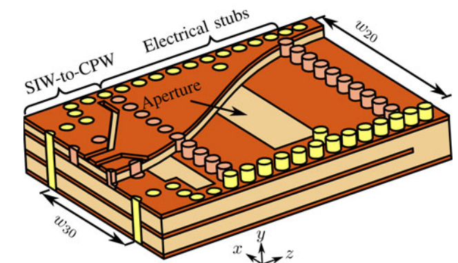
Fig. 5. Model of the diplexer with two different cutaway views.
