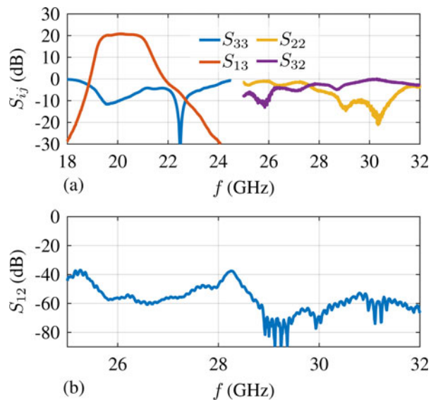
Fig. 16. Measured results of the frontend circuit. (a) Transmission and reflection coefficients S_{33} , S_{22} , S_{13} , S_{32} and (b) transmission coefficient S_{12} .
