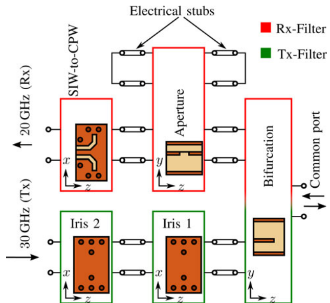
Fig. 6. Schematic representation of the diplexer.
