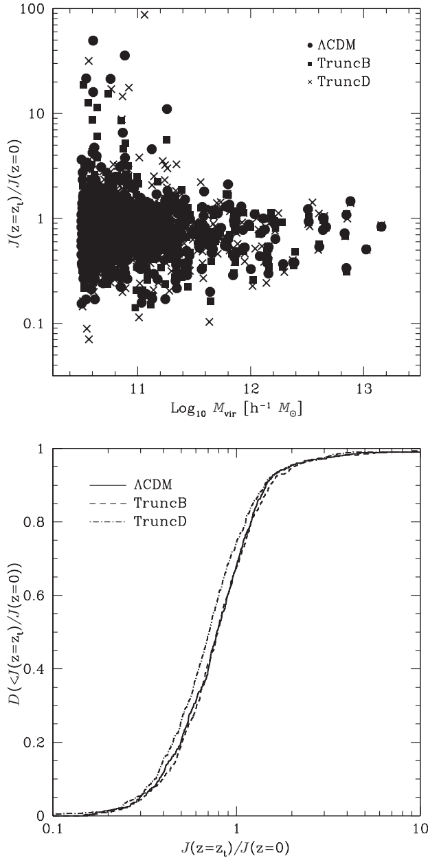
Figure 11. Angular momentum at turnaround. We track the material associated with each halo identified at z=0 and compute the radial extent and angular momentum of this material as a function of redshift in the \Lambda CDM, TruncB, and TruncD runs. When the material has reached its maximum radial extent, we denote the epoch at which this occurs as turnaround and look at the ratio of the magnitude of angular momentum of the material at this redshift z_t , J(z_t) , with respect to the magnitude of the angular momentum of this material at z=0 . In the upper panel, we show the variation of this ratio with halo mass at z=0 ; in the lower panel, we show the cumulative distribution D(<J(z_t)/J(z=0)) .
