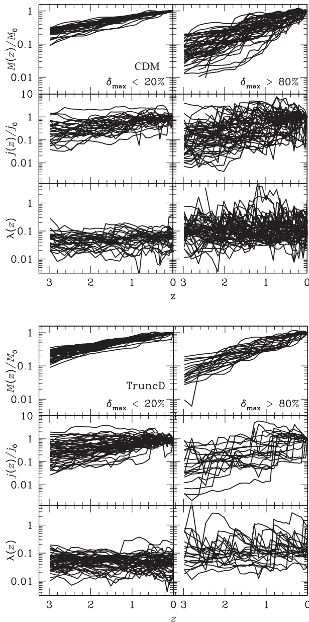
Figure 7. Variation of \lambda and j with redshift for relaxed and unrelaxed haloes. We use the merging histories of haloes to identify two samples of haloes, one with a quiescent merging history ( \delta_{\max} \lesssim 0.2 since z = 3.0 ; left-hand panels) and one with a violent merging history ( \delta_{\max} \gtrsim 0.8 over the same period; right-hand panels) in the \Lambda CDM and TruncD runs (upper and lower panels, respectively). Haloes are chosen such that their virial mass at z = 0 satisfies M_{\text{vir}} \geq 10^{11} h^{-1} M_{\odot} ( \sim 3\,000 particles). The upper, middle, and lower panels show the growth of halo virial mass (normalised to the virial mass at z = 0 ), the specific angular momentum j = J/M (normalised to its value at z = 0 , j_0 ), and dimensionless spin parameter \lambda = JE^{1/2}/GM^{5/2}_{\text{vir}} as a function of redshift z .
