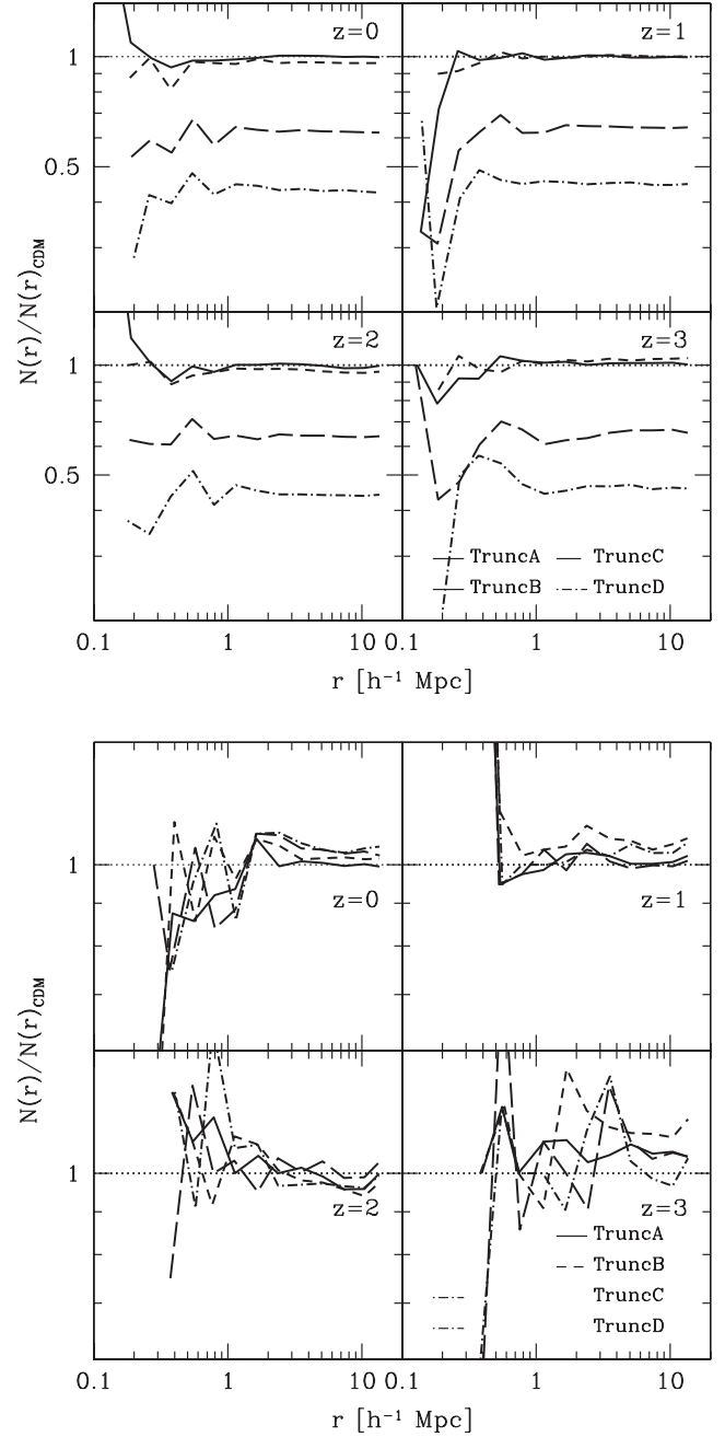
Figure 2. Evolution of spatial clustering with redshift. We examine how the clustering strength of haloes with respect to the fiducial \Lambda CDM model varies across the runs TruncA (solid curves), TruncB (short-dashed curves), TruncC (long-dashed curves), and TruncD (dotted-dashed curves) at z = 0, 1, 2 , and 3 by plotting the ratio N(r)/N(r)_{\text{CDM}} —the number of haloes with comoving halo separation r —as a function of r . In the upper panel, we look at the clustering of all secondary haloes with mass M_{\text{vir}} \geq 3 \times 10^9 h^{-1} M_{\odot} around primary haloes with mass M_{\text{vir}} \geq 10^{11} h^{-1} M_{\odot} , while in the lower panel we look at the clustering of only massive haloes, for which both the primary and secondary masses are M_{\text{vir}} \geq 10^{11} h^{-1} M_{\odot} .
