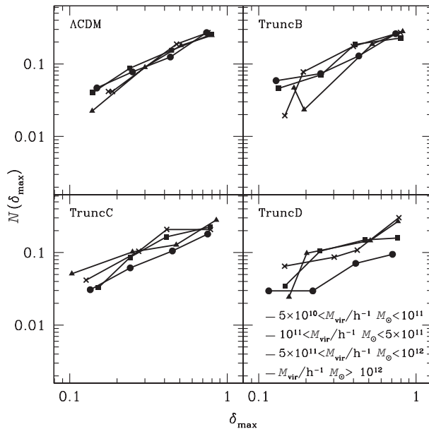
Figure 5. Distribution of most significant mergers. For each halo at z=0 , we compute the mass ratio of the most significant merger \delta_{\text{max}} that it has experienced since z \approx 0.5 and construct the frequency distribution of \delta_{\text{max}} for the respective models.
