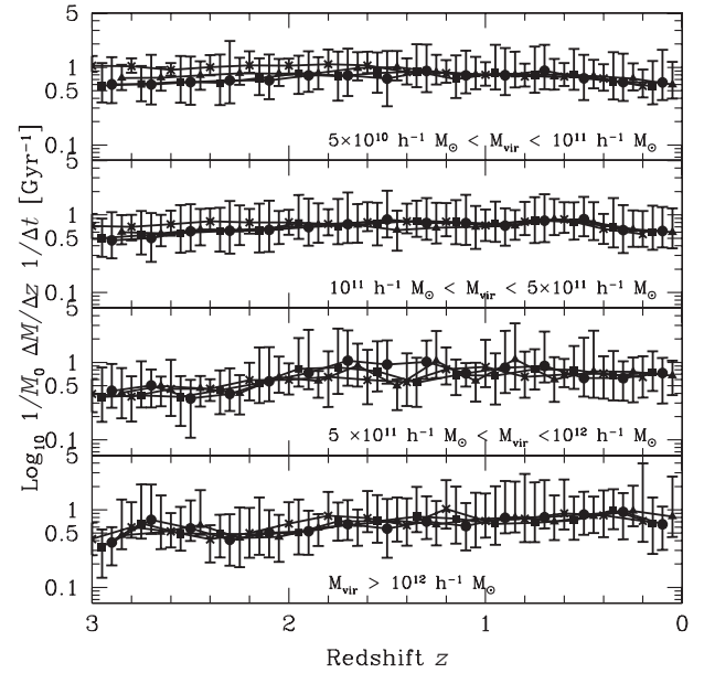
Figure 3. Impact on mass accretion rate. For each halo at z = 0 , we follow the main branch of its merger tree to higher redshifts and compute the difference in virial mass between progenitors at z_0 and z_1 > z_0 . From this, we compute the mass accretion rate with respect to time (in Gyrs), normalised by the virial mass of the descendent halo at z = 0 . Within each of the mass bins, we compute the average mass accretion rate for haloes in the fiducial \Lambda CDM run (red-filled circles), TruncB ( M_{\text{cut}} = 10^{10} h^{-1} M_{\odot} ; green-filled squares), TruncC ( M_{\text{cut}} = 5 \times 10^{10} h^{-1} M_{\odot} ; cyan-filled triangles), and TruncD ( M_{\text{cut}} = 10^{11} h^{-1} M_{\odot} ; magenta crosses).
