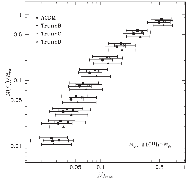
Figure 10. Specific angular momentum profiles. We use the method of Bullock et al. (2001, 2002) to determine the fraction of halo mass that has a total specific angular momentum of j or less. Note that we consider only haloes that satisfy M_{\text{vir}} \geq 10^{11} h^{-1} M_{\odot} .
