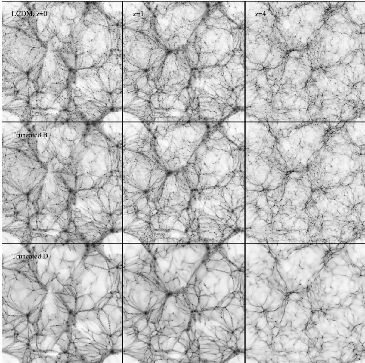
Figure 1. The projected density distribution in 2h^{-1}\text{Mpc} slices taken through the centres of each of the boxes. We have smoothed the particle mass using an adaptive Gaussian kernel and projected onto a mesh. Each mesh point is weighted according to the logarithm of its projected surface density, and so the ‘darker’ the mesh point, the higher the projected surface density.
