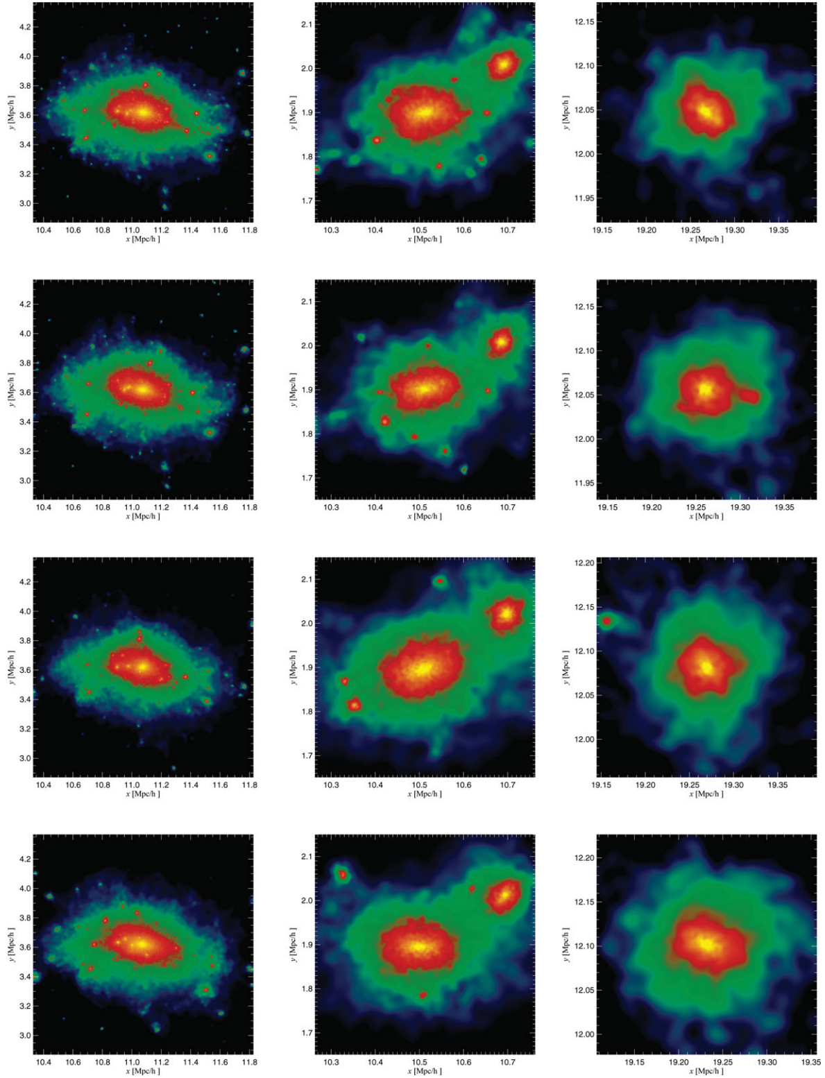
Figure 8. Direct comparison of haloes: projected dark matter density maps. From left to right, haloes with virial masses at z = 0 of M_{\text{vir}} \simeq (7.85, 0.61, 0.076) \times 10^{12} h^{-1} M_{\odot} in the CDM, TruncB, TruncC, and TruncD (from top to bottom).
