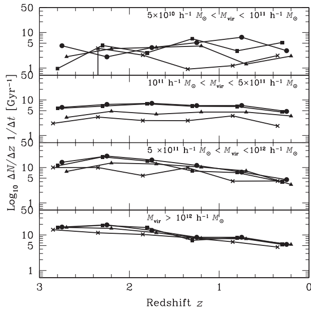
Figure 4. Impact on merger rate. For each halo at z=0 , we follow the main branch of its merger tree to higher redshifts and determine the number of mergers with mass ratios in excess of 6% experienced by the halo between z_0 and z_1 > z_0 . From this, we compute the merger rate per unit redshift per unit time. Within each of the mass bins, we compute the average merger rate for haloes in the fiducial \lambda CDM run (red-filled circles), TruncB ( M_{\text{cut}} = 10^{10} h^{-1} M_\odot ; green-filled squares), TruncC ( M_{\text{cut}} = 5 \times 10^{10} h^{-1} M_\odot ; cyan-filled triangles), and TruncD ( M_{\text{cut}} = 10^{11} h^{-1} M_\odot ; magenta crosses).
