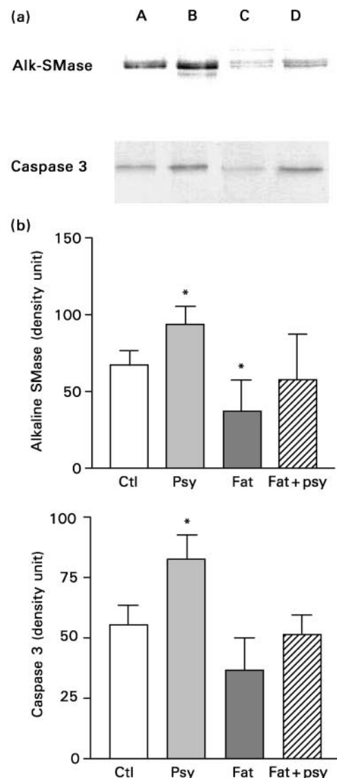
Fig. 3. Expression of alkaline (alk) sphingomyelinase (SMase) and caspase 3 in mice (twelve per group) fed control (Ctl), psyllium-containing (Psy), high-fat (Fat) or high-fat plus psyllium (Fat + psy) diets for 4 weeks. The colonic mucosa was scraped and homogenised. Four animals in each group were randomly selected for Western blotting analysis. In each lane, 50 \mu g sample proteins were loaded. For details of diets and procedures, see Tables 1 and 2 and pp. 716–717. (a), A representative result of Western blotting. Lane A, Ctl; lane B, Psy; lane C, Fat; lane D, Fat + psy. (b), Quantification of the band densities by Scion Image software (Scion Co.; www.scioncorp.com). Values are means with standard deviations shown by vertical bars. Mean values were significantly different from those of the control group: * P < 0.05 .
