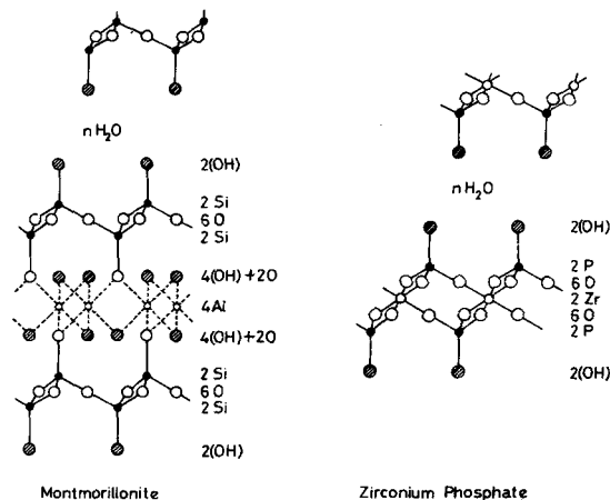
Fig. 1. Schematic presentation of the structure of montmorillonite suggested by Edelman and Favejee, and that of zirconium phosphate.
