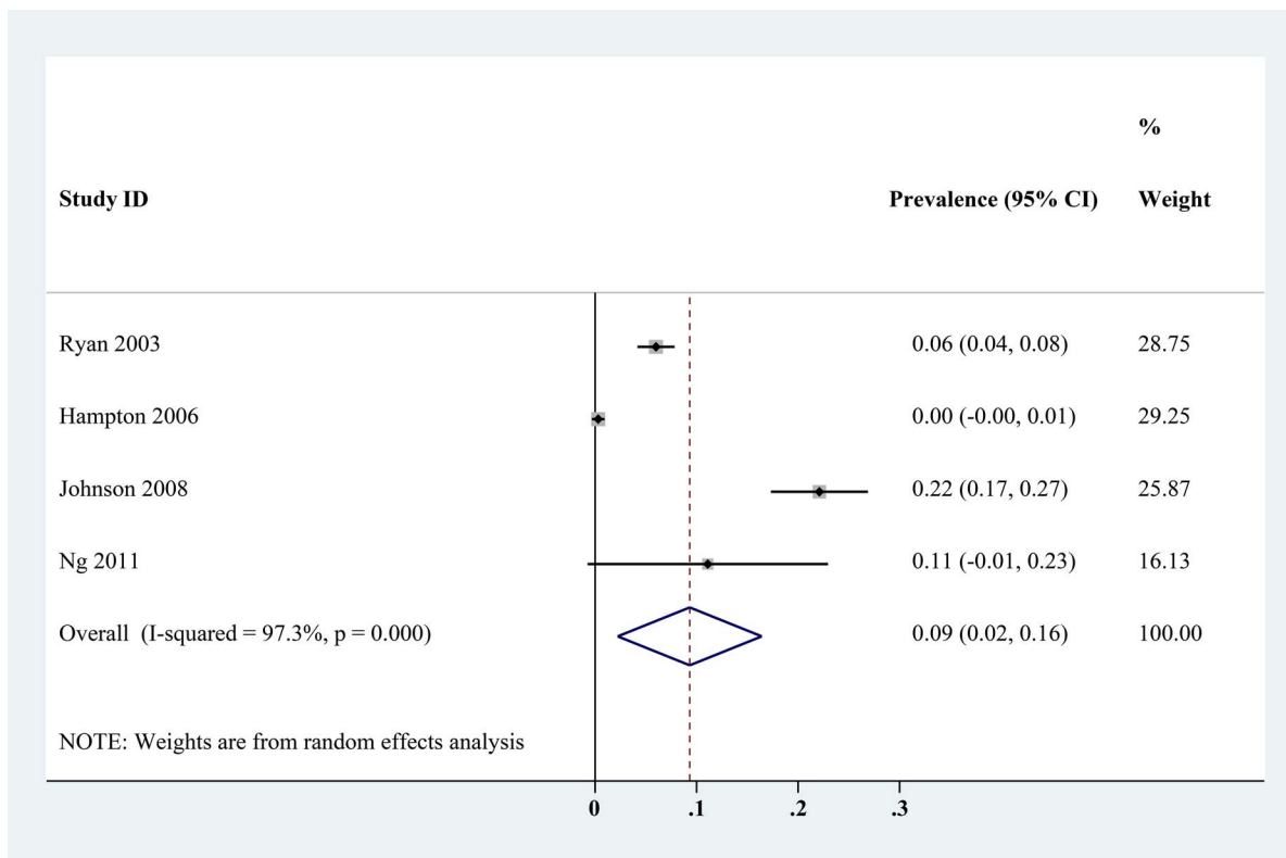
Fig. 8. Forest plot of the prevalence estimates of Cryptosporidium infection in pigs in Oceania.
