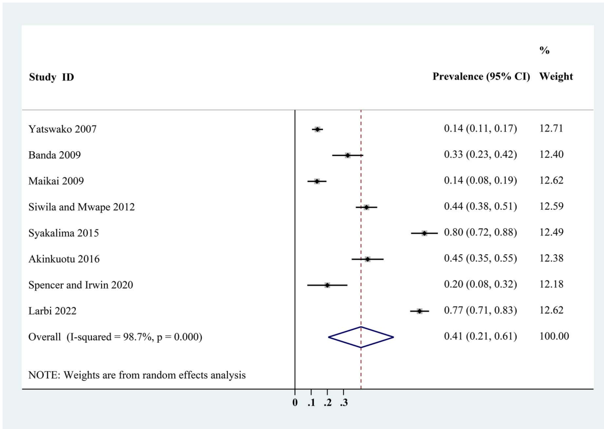
Fig. 5. Forest plot of the prevalence estimates of Cryptosporidium infection in pigs in Africa.
