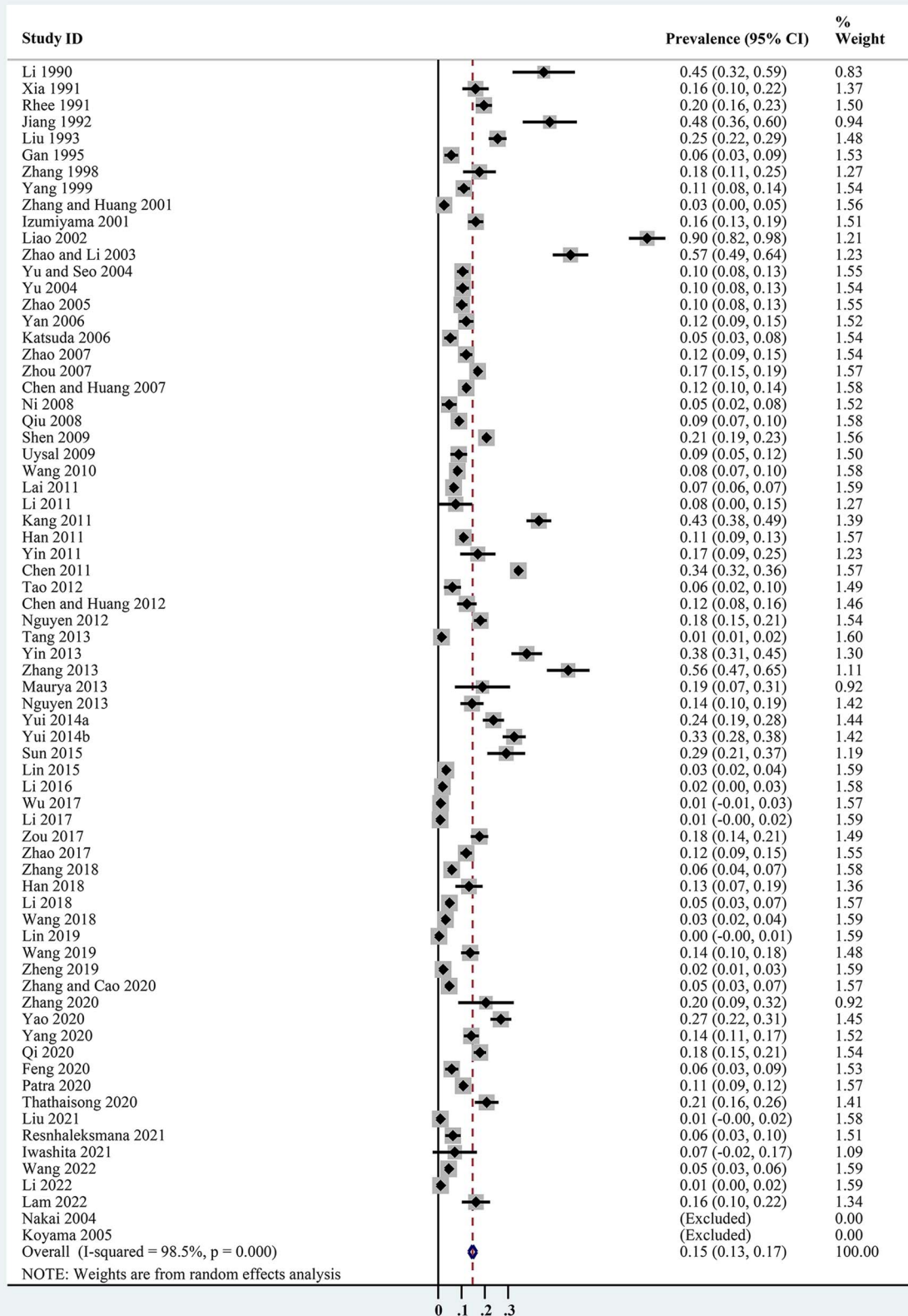
Fig. 3. Forest plot of the prevalence estimates of Cryptosporidium infection in pigs in Asia.
