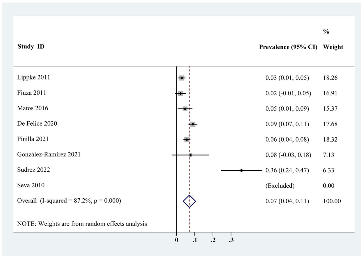
Fig. 7. Forest plot of the prevalence estimates of Cryptosporidium infection in pigs in South America.
