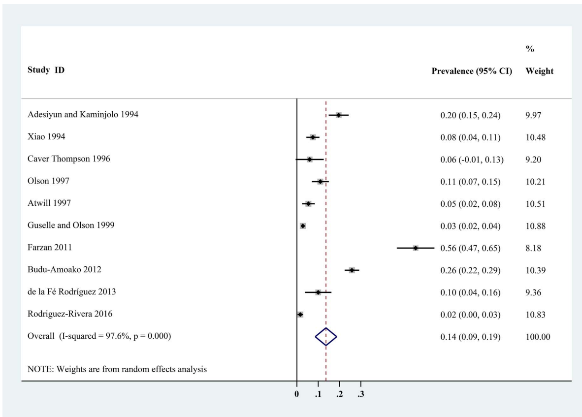
Fig. 6. Forest plot of the prevalence estimates of Cryptosporidium infection in pigs in North America.
