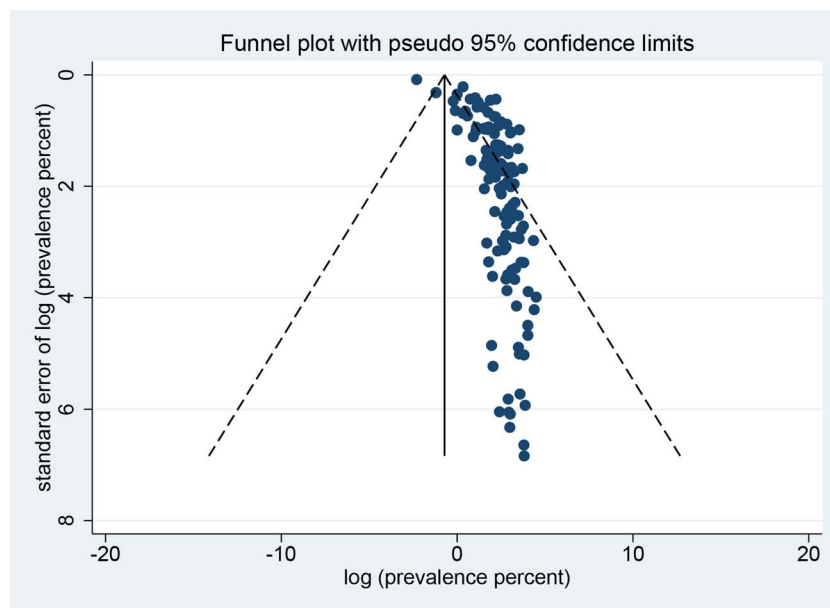
Fig. 9. Funnel plot for examination of publication bias of the prevalence estimates of Cryptosporidium infection in pigs across the world.
