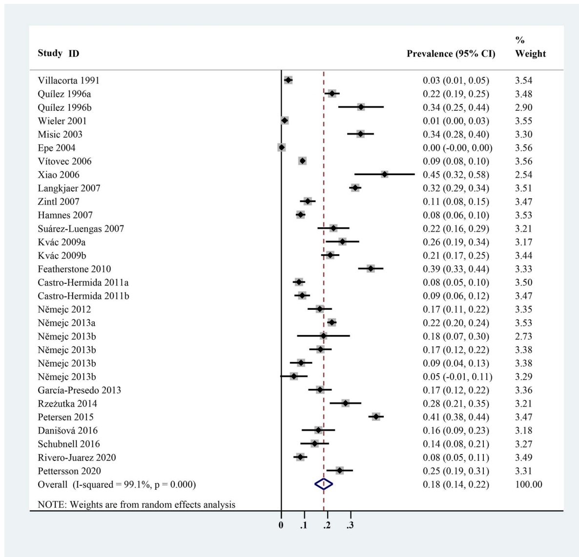
Fig. 4. Forest plot of the prevalence estimates of Cryptosporidium infection in pigs in Europe.
