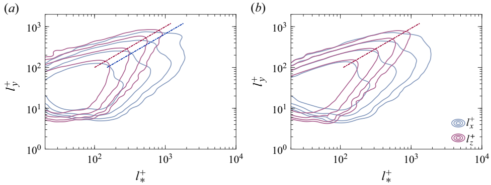
Figure 5. Joint p.d.f.s of the structure height and another dimension for detached (a) intense u' structures and (b) intense T' structures. The red line denotes l_*^+ \approx l_y^+ and the blue line denotes l_*^+ \approx 1.5l_y^+ , where subscript ‘*’ can be x or z . The contour levels are logarithmically distributed.
