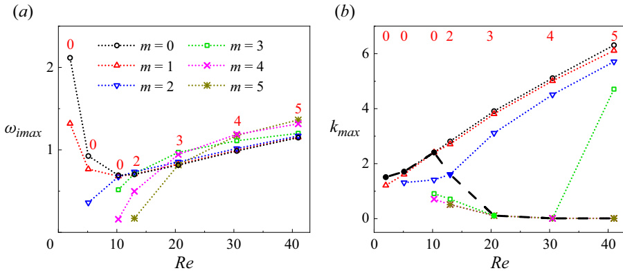
Figure 3. (a) Maximum perturbation growth rate \omega_{imax} for different azimuthal modes as Re varies. (b) Most unstable wavenumber k_{max} for different azimuthal modes as Re varies, where the most unstable wavenumbers corresponding to the predominant mode are depicted by the filled symbols and connected by the black thick dashed line. In both panels, the predominant modes are indicated by red numbers. The other parameters are the same as those in figure 2.
