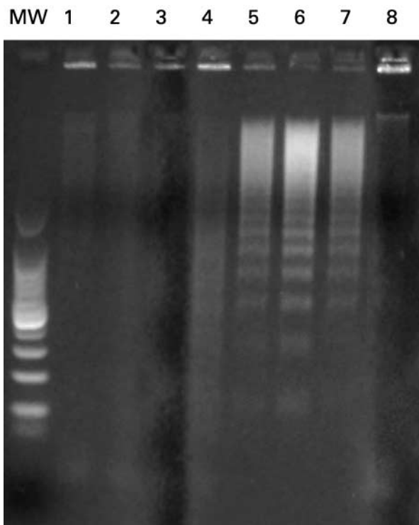
Fig. 5. Induction of DNA fragmentation following a 24 h incubation with \beta -sitosterol oxides and 7 \beta -hydroxycholesterol. DNA fragmentation was assessed by agarose gel electrophoresis. MW, molecular-weight marker; 1, control; 2, 30 \mu M- \beta -sitosterol; 3, 60 \mu M- \beta -sitosterol; 4, 30 \mu M- \beta -sitosterol oxides; 5, 60 \mu M- \beta -sitosterol oxides; 6, 120 \mu M- \beta -sitosterol oxides; 7, 30 \mu M-7 \beta -hydroxycholesterol; 8, 60 \mu M-sitosterol-5 \alpha ,6 \alpha -epoxide.
