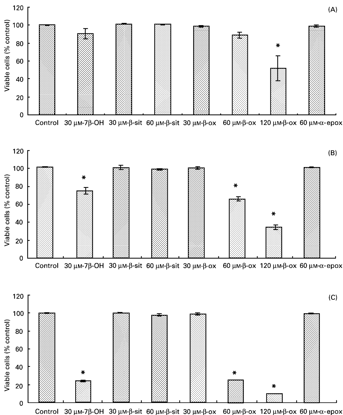
Fig. 3. The viability of U937 cells, expressed as a percentage of control, following a 12 h (A), 24 h (B) and 48 h (C) incubation with 7 \beta -hydroxy-cholesterol (7 \beta -OH), \beta -sitosterol ( \beta -sit), \beta -sitosterol oxides ( \beta -ox) and sitosterol-5 \alpha ,6 \alpha -epoxide ( \alpha -epox). Viability was assessed by the fluorescein diacetate–ethidium bromide membrane permeability assay. Data are mean values for three independent experiments, with the standard errors of the mean represented by vertical bars. *Mean value was significantly different from control ( P < 0.01 ; ANOVA followed by Dunnett's test).
