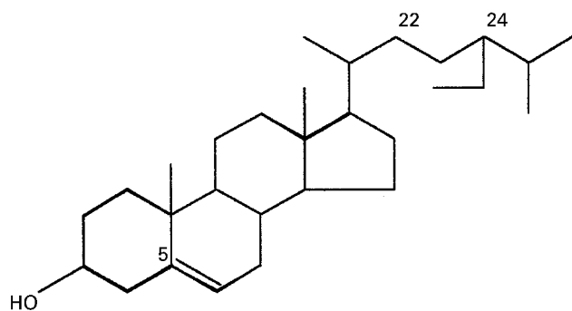
Fig. 1. The chemical structure of \beta -sitosterol.
