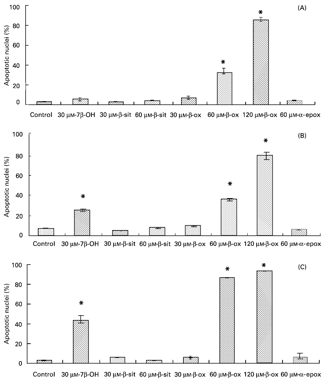
Fig. 4. Condensed and fragmented nuclei, expressed as a percentage of control, following a 12 h (A), 24 h (B) and 48 h (C) incubation with 7 \beta -hydroxycholesterol (7 \beta -OH), \beta -sitosterol ( \beta -sit), \beta -sitosterol oxides ( \beta -ox) and sitosterol-5 \alpha ,6 \alpha -epoxide ( \alpha -epox). Condensed and fragmented nuclei were determined by staining with Hoechst 33342. Data are mean values for three independent experiments, with the standard errors of the mean represented by vertical bars. *Mean value was significantly different from control ( P < 0.01 ; ANOVA followed by Dunnett's test).
