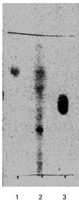
Fig. 2. Oxidation products of \beta -sitosterol observed on silica gel TLC plates developed in diethyl ether using vanilline. 1, \beta -sitosterol; 2, oxidation products of \beta -sitosterol after 48 h heating at 100^\circ\text{C} ; 3, sitosterol- 5\alpha,6\alpha -epoxide.
