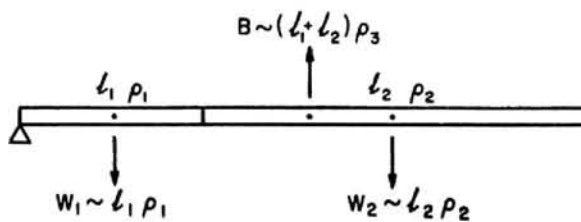
Fig. 2. When the rectifying moment of the buoyant force about the pivot point is greater than the sum of the tilting moments of the various parts, the drill assumes a vertical attitude.
