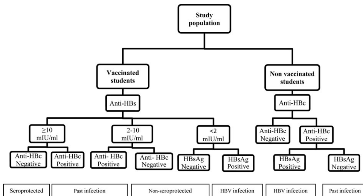
Fig. 1. Study flowchart.
