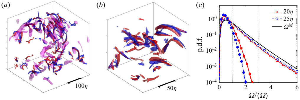
Figure 2. (a) Visualisation of intense vorticity structures in the slave systems ‘A’ (red) and ‘B’ (blue), and of structures of intense vorticity in the large scales of the master system (magenta) for \ell_a = 20\eta . Red and blue isosurfaces (slave systems) correspond to \Omega^{A,B} = 3\langle\Omega\rangle , and magenta isosurfaces (master system) to \Omega_l^M = 4\langle\Omega_l^M\rangle . The panel shows the full computational domain. (b) Detail of the synchronisation of intense vortices in the slave systems in a (150\eta)^3 subdomain. Colours as in panel (a). The data in (a,b) correspond to different flow fields from simulations at Re_\lambda = 120 . (c) Probability density function of the large-scale vorticity magnitude, \Omega_l^A (solid markers), and the small-scale vorticity magnitude, \Omega_s^A (empty markers), in the slave system, and the vorticity magnitude in the master system \Omega^M (solid black line) for Re_\lambda = 120 . All quantities are normalised with \langle\Omega\rangle in each system. Dotted vertical lines mark \Omega/\langle\Omega\rangle = 1 and 3.
