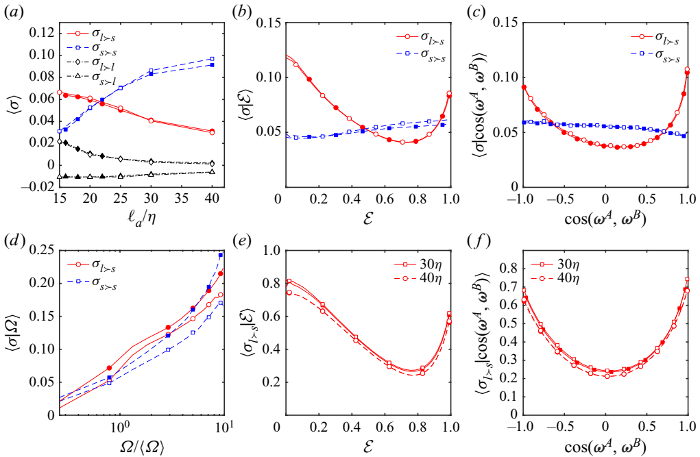
Figure 4. (a) Average amplification of the vorticity magnitude, \sigma_{\alpha>\beta} , due to contributions of the rate-of-strain tensor and the vorticity vector at different scales; see (4.3). (b–d) Average of \sigma_{l>s} and \sigma_{s>s} in the slave systems for \ell_a = 20\eta conditioned to: (b) the error, (c) the angle of alignment and (d) the magnitude of the vorticity vector. In panels (a–d) quantities are normalised with Kolmogorov units. (e, f) Average of \sigma_{l>s} conditioned to: (e) the error and (f) the angle of alignment at different assimilation scales, normalised with the inertial time \tau_a = (\ell_a^2/\langle \varepsilon \rangle)^{1/3} . Empty markers correspond to Re_\lambda = 120 and solid markers to Re_\lambda = 195 .
