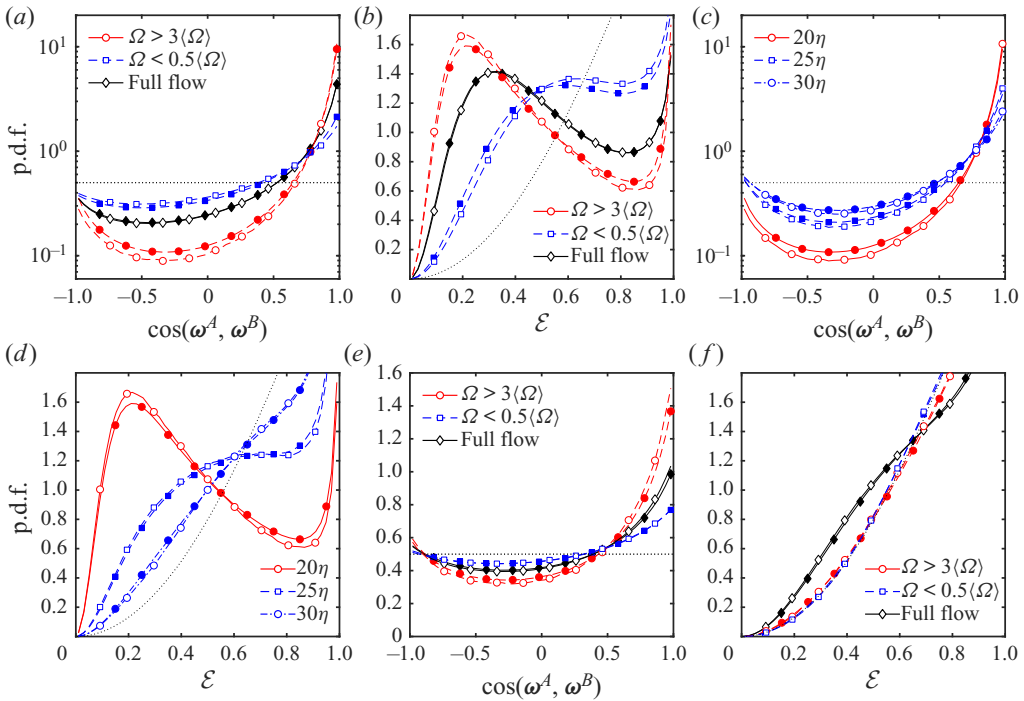
Figure 3. (a,b) The p.d.f.s of (a) the angle of alignment and (b) the error between the vorticity vector of the slave systems as a function of the intensity of the vorticity magnitude for \ell_a = 20\eta . (c,d) The p.d.f.s of (c) the angle of alignment and (d) the error between the vorticity vector of the slave systems for \Omega > 3\langle\Omega\rangle for different assimilation scales. (e,f) The p.d.f.s of (e) the angle of alignment and (f) the error between the vorticity vector of the slave systems as a function of the intensity of the vorticity magnitude for \ell_a = 40\eta . In all panels the empty markers correspond to Re_\lambda = 120 and solid markers to Re_\lambda = 195 . The dotted lines mark the error and angle of alignment of fully decorrelated vorticity fields.
