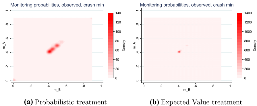
Fig. 6 Officer monitoring probabilities, observed monitoring, crash minimization treatment
