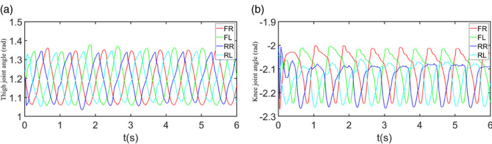
Figure 25. Changes of leg joint angles during the execution of walking gait in the quadruped robot based on GD-CPG. (a) Thigh joint, (b) Knee joint.
