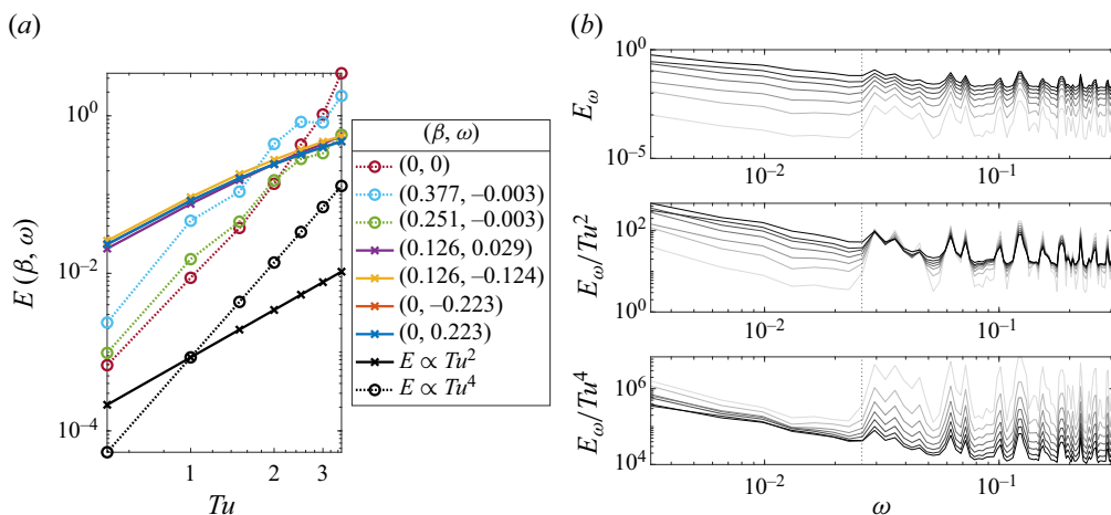
Figure 6. Energy as a function of FST level, Tu . (a) Evolution of most energetic pairs (\beta, \omega) . Legend: (x) linear behaviour; (o) nonlinear behaviour. (b) Normalised energy spectrum. Higher frequencies grow with a Tu^2 dependency, while lower frequencies scale with a factor closer to Tu^4 . Darker lines indicate higher FST levels. The vertical line, drawn at \omega = 0.026 , separates higher- and lower-frequency ranges.
