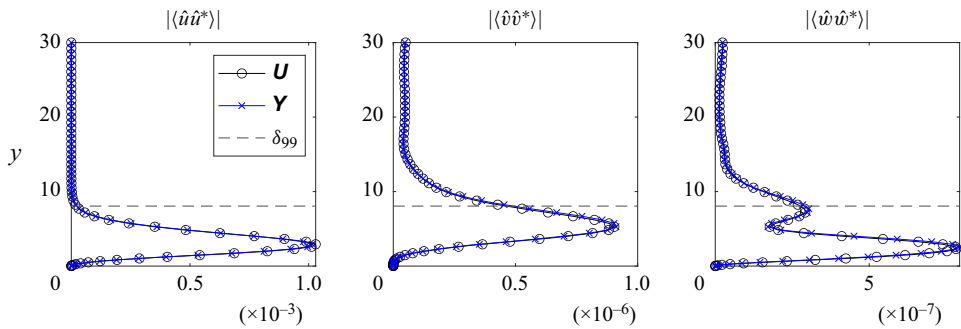
Figure 28. Comparison between mean-squared velocities computed from LES statistics, \mathbf{U} , and reconstructed statistics, \mathbf{Y} , at (\beta, \omega) = (0.377, -0.003) , Tu = 3.5\% and x = 700 . Respectively, \langle \cdot \rangle , |\cdot| and \{\cdot\}^* are averages over blocks, absolute value and conjugate.
