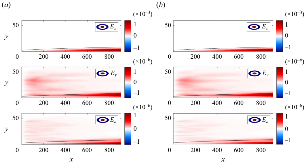
Figure 27. Computed PSDs at (\beta, \omega) = (0.377, -0.003) and Tu = 3.5\% . (a) Statistical PSD, P_U and (b) reconstructed PSD, P_Y .
