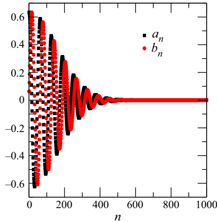
Figure 4. Spectral coefficients a_n and b_n for k_e = 0.05i and Pe = 10^6 and t \rightarrow \infty . The spectral coefficients are truncated at n = 1000 , since a_n, b_n \rightarrow 0 above this threshold.
