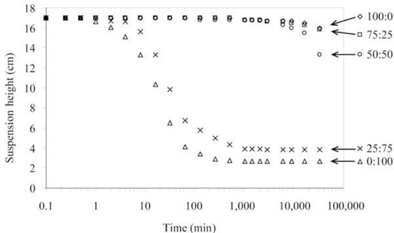
Figure 9. Controlling particle interaction through changes in surface chemistry: sedimentation curves for Premier-PCC mixtures.
