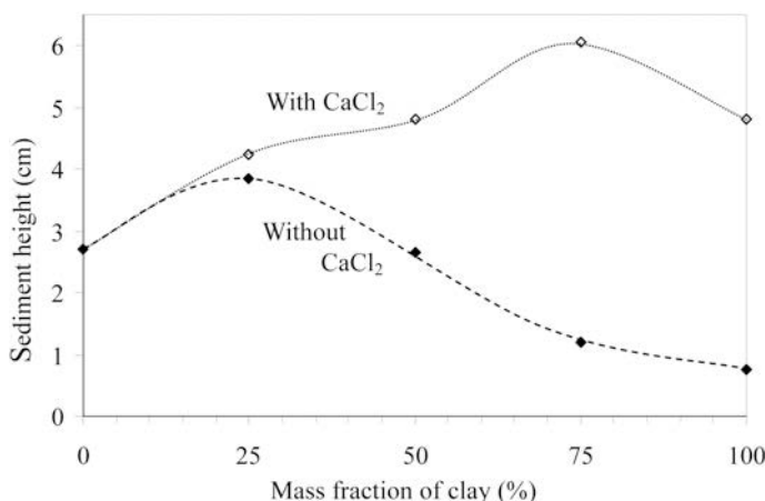
Figure 10. Controlling particle interaction through changes in surface chemistry and pore fluid. Final sediment height at 23 days for Premier-PCC mixtures with and without CaCl 2 .
