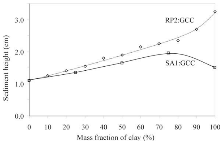
Figure 8. The effect of relative geometry on the 273 H sediment height of dilute suspensions. The mixtures were prepared with the same carbonate GCC, but with different kaolinities: RP2, SA1. The sediment height is determined at the sediment-suspension interface.
