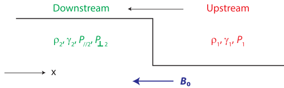
FIGURE 1. Densities \rho_i and pressures P_i are measured in the fluids (upstream and downstream) rest frame. Lorenz factors \gamma_i are measured in the front frame. The upstream is assumed isotropic, but not the downstream. Only the case of a strong shock, namely P_{\perp 1} = 0 (sonic Mach number M_s = \infty ) and \gamma_1 \gg 1 , is studied in this work.
