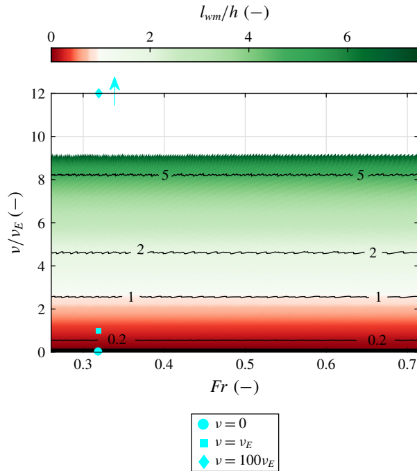
FIGURE 4. (Colour online) Wavelength of the shortest perturbation with positive growth rate ( l_{wm} ) relative to the flow depth ( h ) as a function of the Froude number ( Fr ) and the diffusion coefficient ( v ) relative to the diffusion coefficient according to Elder (1959) ( v_E ). Different flow conditions are studied varying the flow depth between 0.2 m and 1.5 m from the reference case (table 1). The cyan markers indicate the conditions of three numerical simulations with different values of the diffusion coefficient (§ 5.1). The arrow next to the diamond marker indicates that the value lies outside the figure. Red (green) colour indicates that the shortest wavelength with positive growth rate are smaller (larger) than the flow depth.
