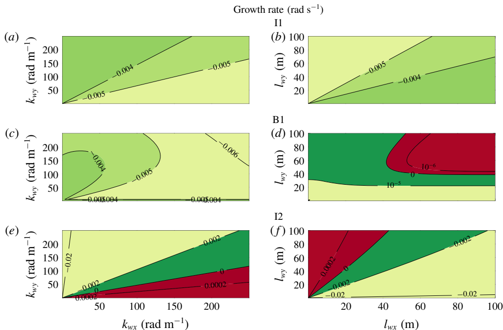
FIGURE 1. (Colour online) Growth rate of perturbations added to the reference case (tables 1 and 2) as a function of the wavenumber and the wavelength: (a–b) iSWE, Fr < 2 (Case I1, well posed), (c–d) iSWE+Exner (Case B1, well posed) and (e–f) iSWE, Fr > 2 (Case I2, ill posed). The panels in the two columns show the same information but highlight the behaviour for large wavenumbers (left column) and for large wavelengths (right column). Red and green indicates growth and decay of perturbations, respectively.
