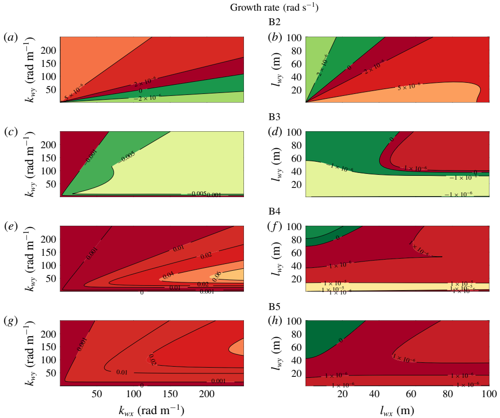
FIGURE 5. (Colour online) Growth rate of perturbations added to the reference case (tables 1 and 5) as a function of the wavenumber and the wavelength: (a,b) Case B2 (ill posed), (c,d) Case B3 (well posed), (e,f) Case B4 (ill posed) and (g,h) Case B5 (ill posed). The panels in the two columns show the same information but highlight the behaviour for large wavenumbers (a,c,e,g) and for large wavelengths (b,d,f,h). Red and green indicate growth and decay of perturbations, respectively.
