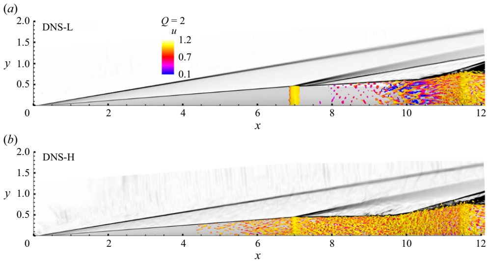
Figure 8. Comparison of instantaneous flow features for (a) DNS-L and (b) DNS-H shown via 100 equally spaced contours of |\nabla\rho| between 0 and 10. Vortical structures in the flow are shown via isolevels of Q -criterion = 2, coloured by streamwise velocity.
