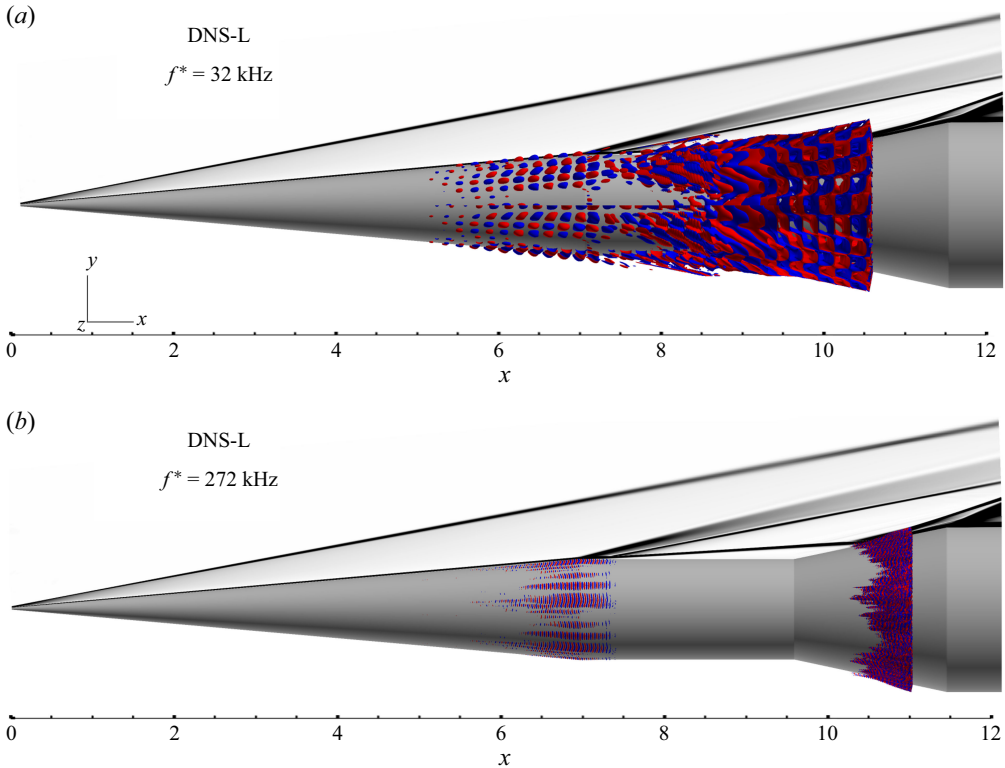
Figure 14. Dominant SPOD mode of pressure fluctuations at two frequencies: (a) f^* = 32 kHz and (b) f^* = 272 kHz corresponding to Mack's first and second modes, respectively, obtained from DNS-L. Isolevels of pressure fluctuations = \pm 0.2 are used to visualize the modes. Mean flow features are shown via 100 equally spaced contours of |\nabla \rho| between 0 and 10.
