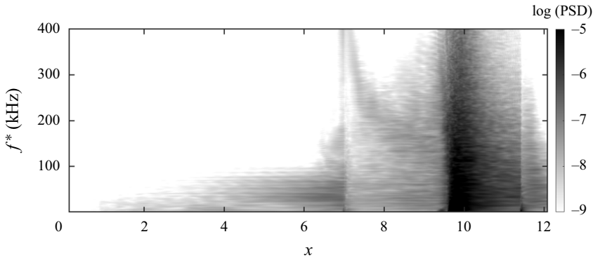
Figure 17. Streamwise variation of wall pressure spectra obtained from DNS-H.
