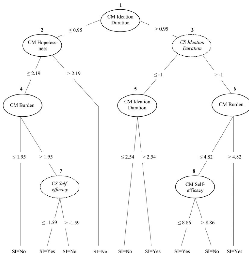
Fig. 1. Prediction rule for next-day suicidal ideation. Notes: SI = Next-day suicidal ideation; CM = Cumulative person-specific mean; CS = Change score (deviation from the person-specific mean); Bolded numbers are added to denote nodes for ease of interpretation (see Table 2 for interpretation).
