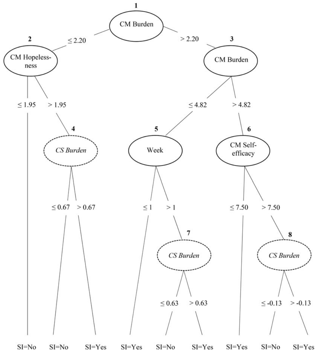
Fig. 2. Prediction rule for next-day suicidal ideation excluding previous-day ideation duration.
