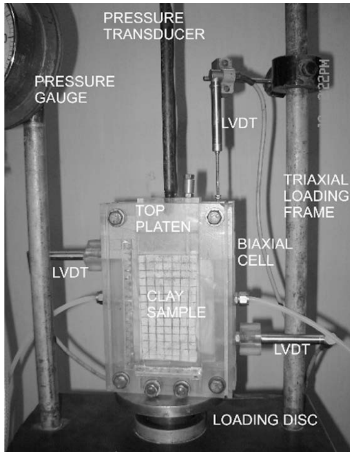
Figure 4. Details of the biaxial cell and biaxial test setup. The kaolinite matrix with imprinted 10 mm \times 10 mm grids on it can be seen through the transparent perspex sheet in front of the cell. The LVDTs attached to the sample measure deformation in the vertical and the two free lateral directions. The kaolinite sample is sheared under compressive load imparted by raising the loading disk at the bottom at a constant rate.
