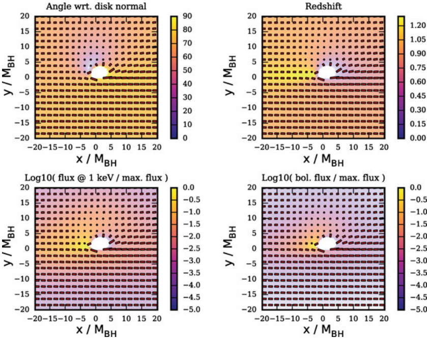
Figure 2. Ray-traced images of a Kerr black hole with a mass of M = 10M_{\odot} , accretion rate of \dot{M} = 0.1\dot{M}_{\text{Edd}} and a dimensionless spin of a/M = 0.998 . The surrounding accretion disc is optically thick and geometrically thin, modelled with the Novikov–Thorne equations (Novikov & Thorne 1973). The emission is modelled with a semi-infinite electron scattering atmosphere (Chandrasekhar 1960). The direction of linear polarization is shown by the red bars, and the degree of polarization is indicated by the bar lengths, with the bottom edges corresponding to \sim 4\% . Top left: The angle between the geodesic and the disc normal as measured by an observer co-moving with the disc matter. Top right: The redshift factor, \mathcal{G} , between the disc matter and the observation point. Bottom left: Observed flux at 1 keV, integrated over a 10 keV window, relative to the maximum flux, in logarithmic units. Bottom right: Observed bolometric flux, relative to the maximum flux, in logarithmic units.
