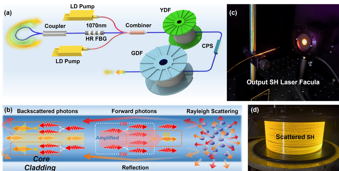
Figure 1. (a) Experimental setup. LD pump, laser diode pump; HR FBG, high-reflection fiber Bragg grating; YDF, ytterbium-doped fiber; GDF, germanium-doped fiber; CPS, cladding power stripper. (b) Principle of SH gain and feedback. (c) Output SH laser facula after a cladding light stripper attached to the output. (d) GDF glowing visible light while the pump is injected.
