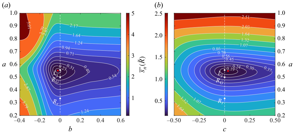
Figure 7. Average standard deviation of the cone-jet radius in 0 \leq \tilde{x} \leq 2\overline{L}_{90} , as a function of the powers in the scaling (a) L_r = L_x = l_o \Pi Q^a Re^b , combined effects of the dimensionless flow rate and Reynolds number; and (b) L_r = L_x = l_o \Pi Q^a \varepsilon^c , combined effects of the dimensionless flow rate and dielectric constant.
