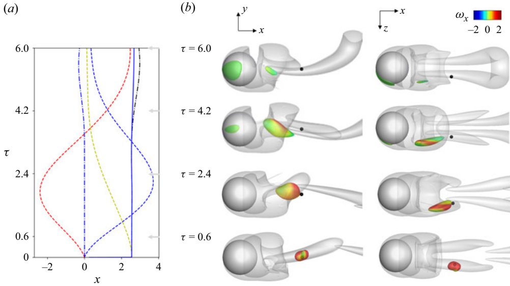
Figure 14. (a) Time history of the terms in the duality relation: (—) \mathcal{I} + \mathcal{B} , (---) \mathcal{I} , (-·-·) \mathcal{B} , (- - -) \mathcal{I}_x , (- - -) \mathcal{I}_r , (- - -) \mathcal{I}_\varphi . (b) Vortical structures visualised using translucent iso-surfaces of Q = 0.2 . The opaque surfaces correspond to the iso-level of the interior contribution, \boldsymbol{\Omega}^x \cdot \boldsymbol{\omega} = 20 , and are coloured by \omega_x . From bottom to top, the panels correspond to the reverse times \tau = \{0.6, 2.4, 4.2, 6.0\} .
