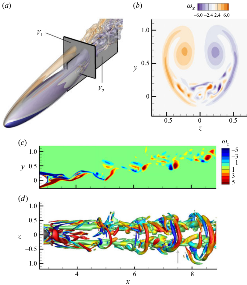
Figure 25. (a) Vortical structures around and in the wake of the prolate spheroid. Translucent surfaces are Q = 2 , coloured by \omega_x . Two visualisation planes, V_1 and V_2 , are marked. (b) Contours of \omega_x on V_1 . (c) Contours of \omega_z on V_2 which is aligned with the x - y plane. (d) Bottom view of the near wake, showing the iso-surface Q = 2 coloured by \omega_z . The grey arrow points to the target necklace vortex whose history will be analysed. Panels (c) and (d) share the same x range.
