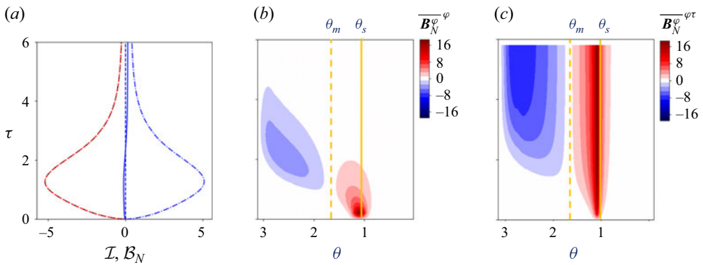
Figure 11. (a) Time histories of the terms in the duality relation, including (—) \mathcal{I} + \mathcal{B}_N , (---) \mathcal{I} , (---) \mathcal{B}_N , (---) \mathcal{I}_x , (---) \mathcal{I}_r , (---) \mathcal{I}_\varphi . Panels (b) and (c) are instantaneous and time-integrated boundary terms, \overline{B}_N^\varphi(\theta, \tau) and \overline{B}_N^{\varphi\tau}(\theta, \tau) . The angles \theta_m and \theta_s correspond to the pressure minimum and separation.
