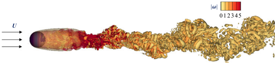
Figure 1. Flow over a fixed body. The free-stream velocity is U . Iso-surfaces of the Q-criterion, Q = 0.1 , show the abundance of vortical structures. Colour shows the magnitude of vorticity.
