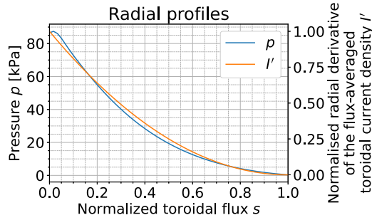
FIGURE 3. Radial profile of pressure p and the normalised radial derivative of the flux-averaged toroidal current density I' = 1 - 2s + s^2 , where s is the normalised toroidal magnetic flux.
