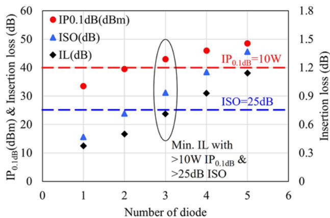
Figure 9. Simulation of the SPDT switch's IP_{0.1 \text{ dB}} , ISO and IL in different numbers of series diodes.
