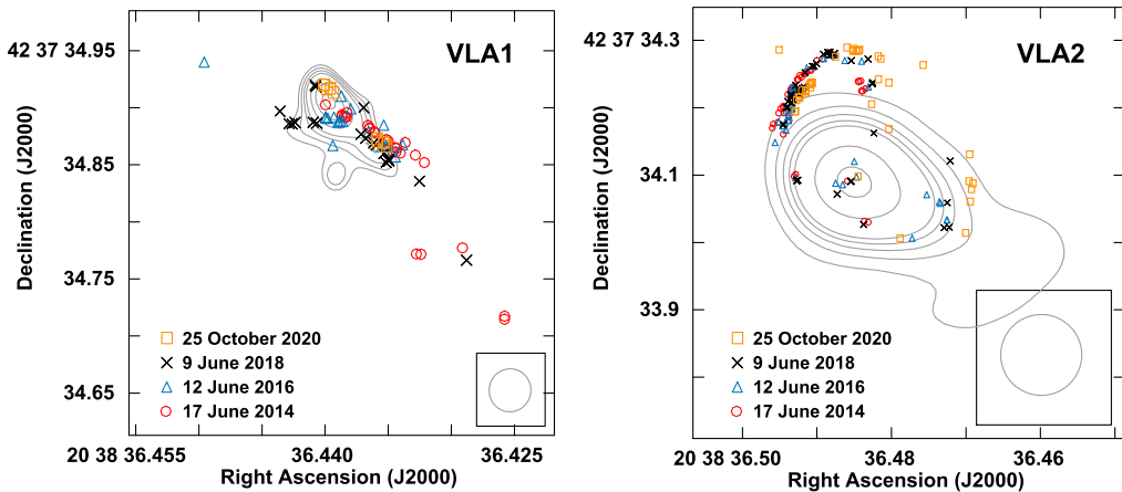
Figure 1. Comparison of the \text{H}_2\text{O} maser features detected toward VLA 1 (left panel) and VLA 2 (right panel) in the four EVN epochs and superimposed to the uniform-weighted continuum map at Q-band (Rodríguez-Kamenetzky et al. 2020) and to the natural-weighted continuum map at K-band (Carrasco-González et al. 2015), respectively, obtained both with the VLA. The light gray contours are 5, 6, 7, 8, 10, 12, 14 times \sigma = 100 \mu\text{Jy beam}^{-1} in the case of VLA 1 and 5, 10, 15, 20, 25, 50, and 75 times \sigma = 10 \mu\text{Jy beam}^{-1} in the case of VLA 2. The VLA beam is shown on the bottom right corner of both panels. The size of the symbols are ten times the uncertainties of the absolute positions of the maser features (see Table 2 of Surcis et al. 2023). For more details see Surcis et al. (2023).
