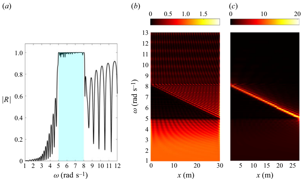
Figure 13. (a) Amplitude of the reflection coefficient |R| for the finite-size floating metaplate with the graded resonant frequencies ranging from 5 to 8 \text{ rad s}^{-1} . (b) Displacement field of the plate and (c) the resonators at different frequencies, illustrating the rainbow reflection effect. Panels (b) and (c) are the same as figure 10, except that the frequency range associated with the rainbow reflection shifted to the new frequency range of the graded resonators.
