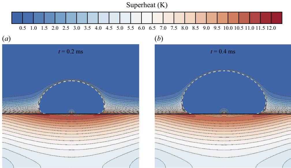
Figure 8. Superheat distributions at (a) t = 0.2 \text{ ms} and (b) t = 0.4 \text{ ms} for case A ( \omega = 0.0345 ), obtained at grid level 12. The white dashed line and the black solid line represent the liquid–vapour interface and the fluid–solid boundary, respectively. The results are mirrored about r = 0 for better visualisation.
